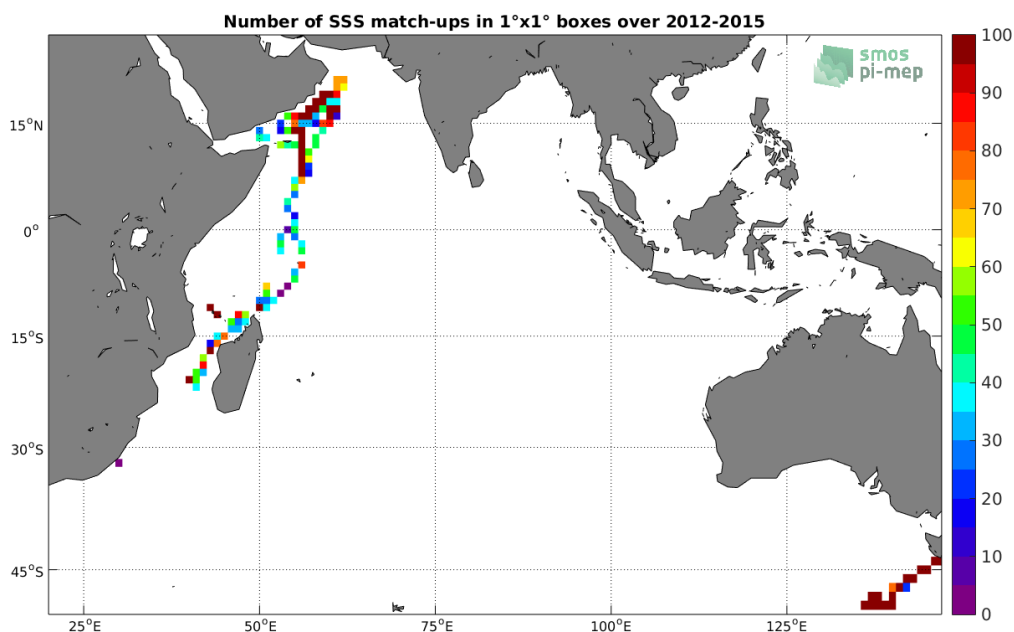
Figure 4: Number of SSS match-ups between TSG-GOSUD-Research-vessel SSS and the Aquarius-L3-JPL-V5-7DAY-RUNNING SSS product for the Indian Ocean Pi-MEP region over 1°x1° boxes and for the full satellite product period.
