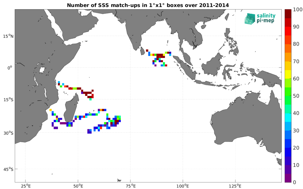
Figure 3: Number of SSS match-ups between Surface drifters SSS and the Aquarius SSS L3 CAP v5 - 7-Day running (JPL) SSS product for the Indian Ocean Pi-MEP region over 1^\circ \times 1^\circ boxes and for the full satellite product period.
