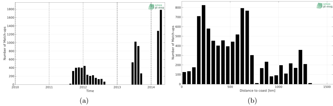
Figure 1: Number of match-ups between Surface drifters and Aquarius SSS L3 CAP v5 - 7-Day running (JPL) SSS as a function of time (a) and as function of the distance to coast (b) over the Indian Ocean Pi-MEP region and for the full satellite product period.
