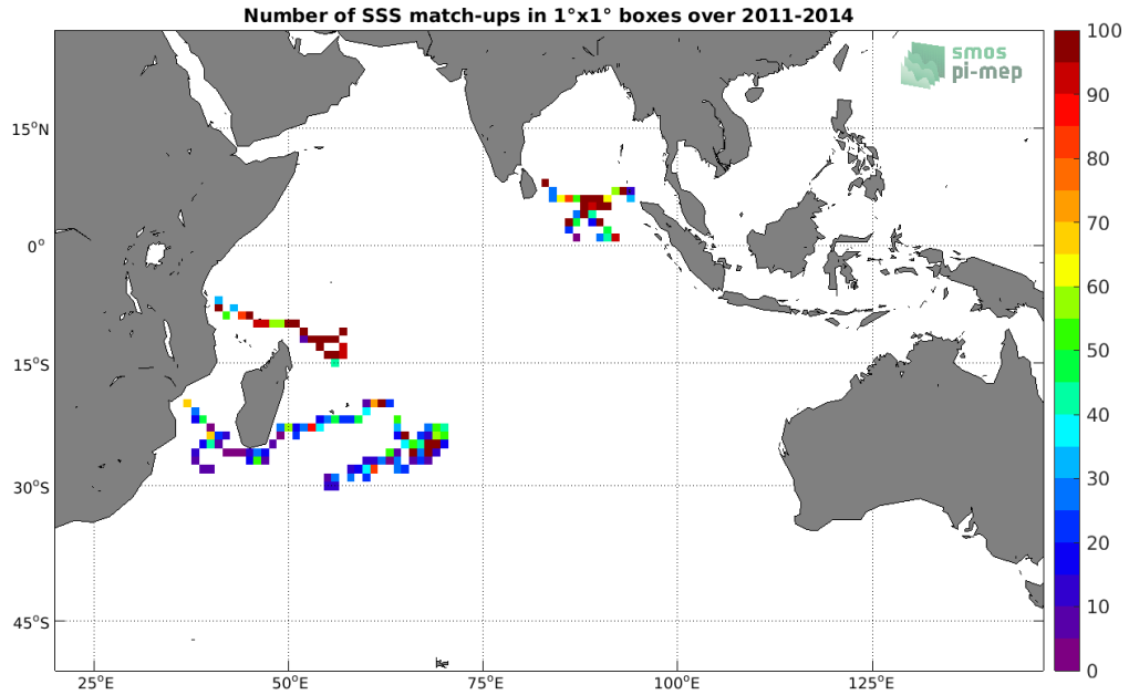
Figure 3: Number of SSS match-ups between Surface drifters SSS and the Aquarius SSS L3 CAP v5 - 7-Day running (JPL) SSS product for the Indian Ocean Pi-MEP region over 1°x1° boxes and for the full satellite product period.
