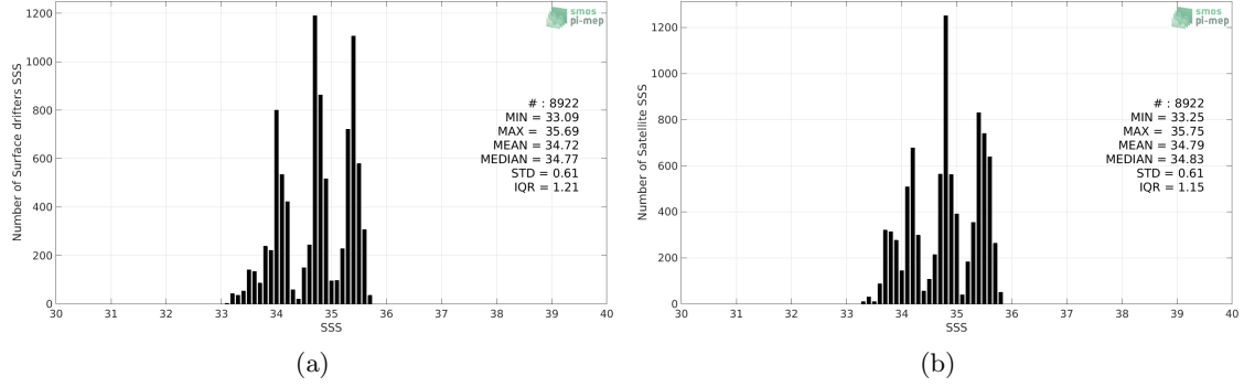
Figure 2: Histograms of SSS from Surface drifters (a) and Aquarius SSS L3 CAP v5 - 7-Day running (JPL) (b) considering all match-up pairs per bins of 0.1 over the Indian Ocean Pi-MEP region and for the full satellite product period.
