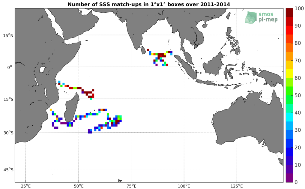
Figure 3: Number of SSS match-ups between Surface drifters SSS and the Aquarius-L3-JPL-V5-7DAY-RUNNING SSS product for the Indian Ocean Pi-MEP region over 1°x1° boxes and for the full satellite product period.
