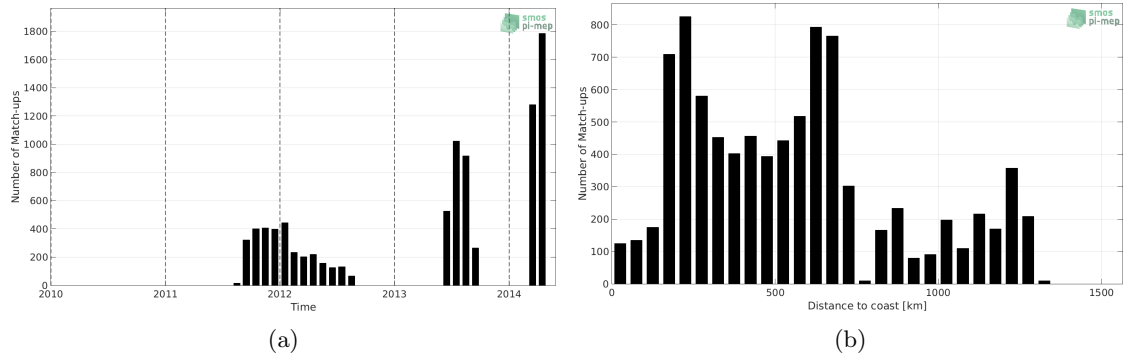
Figure 1: Number of match-ups between Surface drifters and Aquarius-L3-JPL-V5-7DAY-RUNNING SSS as a function of time (a) and as function of the distance to coast (b) over the Indian Ocean Pi-MEP region and for the full satellite product period.
