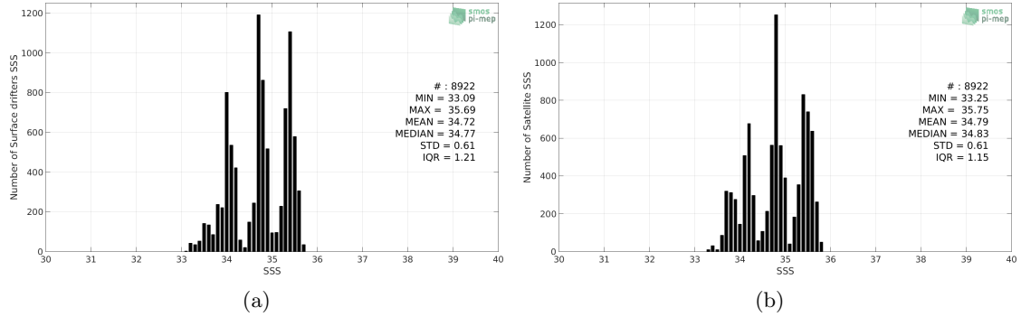
Figure 2: Histograms of SSS from Surface drifters (a) and Aquarius-L3-JPL-V5-7DAY-RUNNING (b) considering all match-up pairs per bins of 0.1 over the Indian Ocean Pi-MEP region and for the full satellite product period.
