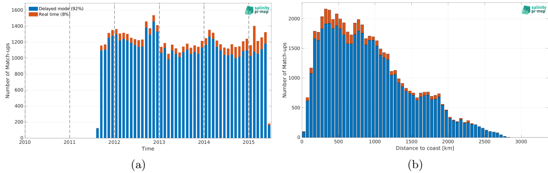
Figure 2: Number of match-ups between Argo and Aquarius SSS L3 CAP v5 - 7-Day running (JPL) SSS as a function of time (a) and as function of the distance to coast (b) over the Indian Ocean Pi-MEP region and for the full satellite product period.
