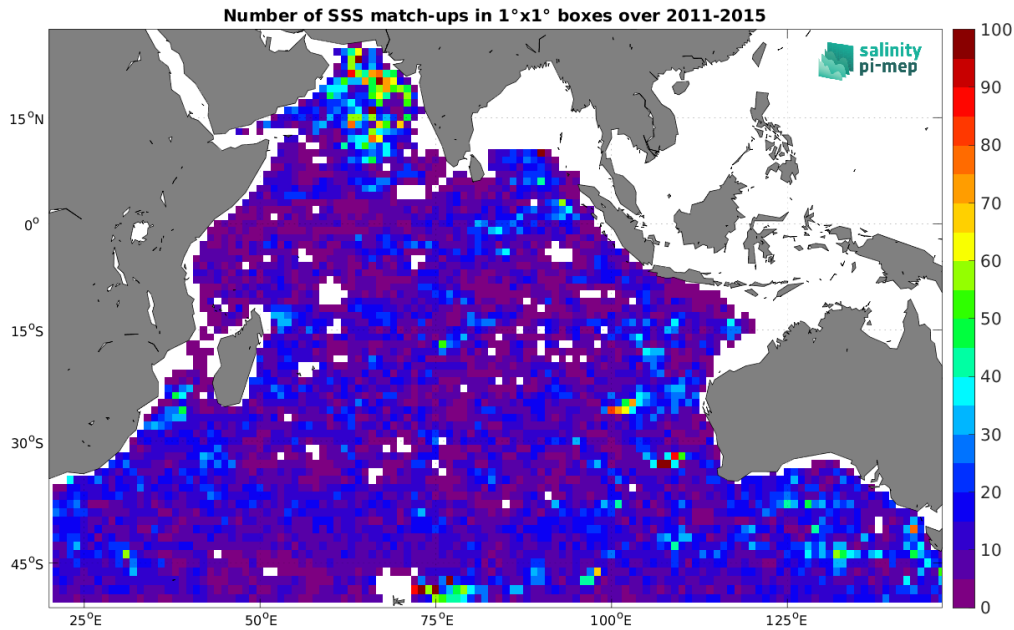
Figure 5: Number of SSS match-ups between Argo SSS and the Aquarius SSS L3 CAP v5 - 7-Day running (JPL) SSS product for the Indian Ocean Pi-MEP region over 1^\circ \times 1^\circ boxes and for the full satellite product period.
