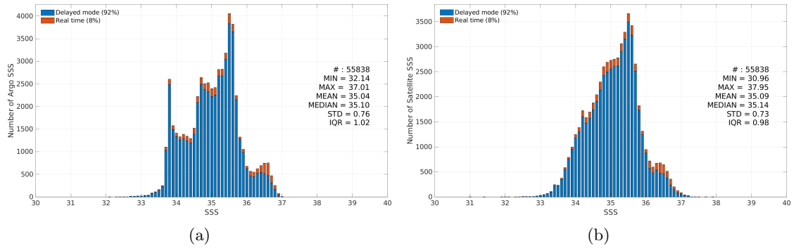
Figure 3: Histograms of SSS from Argo (a) and Aquarius SSS L3 CAP v5 - 7-Day running (JPL) (b) considering all match-up pairs per bins of 0.1 over the Indian Ocean Pi-MEP region and for the full satellite product period.
