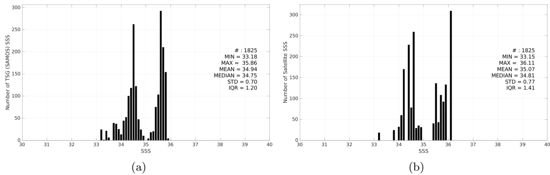
Figure 3: Histograms of SSS from TSG (SAMOS) (a) and Aquarius SSS L3 CAP v5 - Monthly (JPL) (b) considering all match-up pairs per bins of 0.1 over the Indian Ocean Pi-MEP region and for the full satellite product period.
