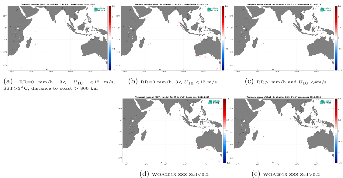
Figure 14: Temporal mean gridded over spatial boxes of size 1^\circ \times 1^\circ of \Delta SSS (Aquarius SSS L3 CAP v5 - Monthly (JPL) - TSG (SAMOS)) for 5 different subdatasets corresponding to:RR=0 mm/h, 3 < U_{10} < 12 m/s, SST >5^\circ\text{C} , distance to coast > 800 km (a), RR=0 mm/h, 3 < U_{10} < 12 m/s (b), RR >1 mm/h and U_{10} < 4 m/s (c), WOA2013 SSS Std <0.2 (d), WOA2013 SSS Std >0.2 (e).
