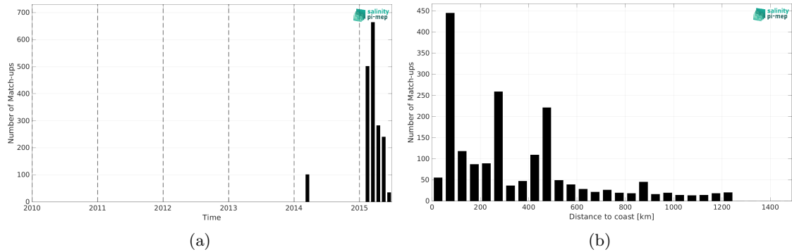
Figure 2: Number of match-ups between TSG (SAMOS) and Aquarius SSS L3 CAP v5 - Monthly (JPL) SSS as a function of time (a) and as function of the distance to coast (b) over the Indian Ocean Pi-MEP region and for the full satellite product period.
