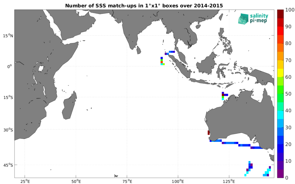
Figure 4: Number of SSS match-ups between TSG (SAMOS) SSS and the Aquarius SSS L3 CAP v5 - Monthly (JPL) SSS product for the Indian Ocean Pi-MEP region over 1^\circ \times 1^\circ boxes and for the full satellite product period.
