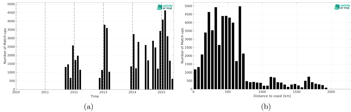
Figure 2: Number of match-ups between TSG (LEGOS-DM) and Aquarius SSS L3 CAP v5 - Monthly (JPL) SSS as a function of time (a) and as function of the distance to coast (b) over the Indian Ocean Pi-MEP region and for the full satellite product period.
