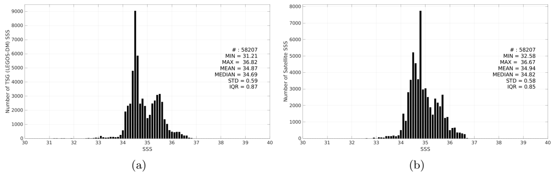
Figure 3: Histograms of SSS from TSG (LEGOS-DM) (a) and Aquarius SSS L3 CAP v5 - Monthly (JPL) (b) considering all match-up pairs per bins of 0.1 over the Indian Ocean Pi-MEP region and for the full satellite product period.
