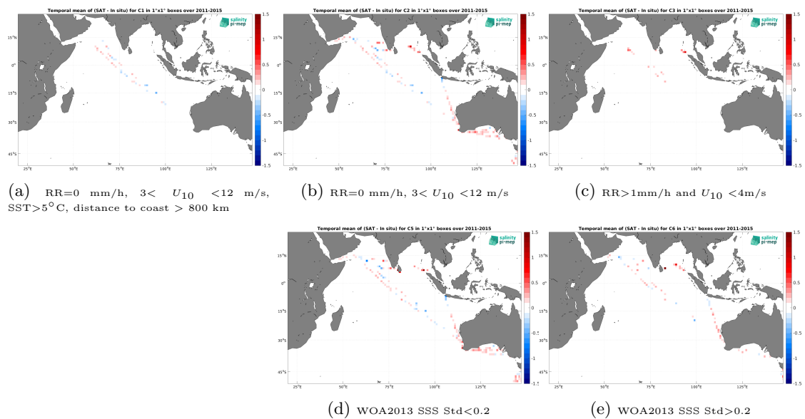
Figure 14: Temporal mean gridded over spatial boxes of size 1^\circ \times 1^\circ of \Delta SSS (Aquarius SSS L3 CAP v5 - Monthly (JPL) - TSG (LEGOS-DM)) for 5 different subdatasets corresponding to: RR=0 mm/h, 3 < U_{10} < 12 m/s, SST > 5^\circ\text{C} , distance to coast > 800 km (a), RR=0 mm/h, 3 < U_{10} < 12 m/s (b), RR > 1 mm/h and U_{10} < 4 m/s (c), WOA2013 SSS Std < 0.2 (d), WOA2013 SSS Std > 0.2 (e).
