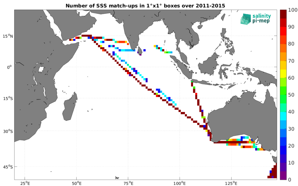
Figure 5: Number of SSS match-ups between TSG (LEGOS-DM) SSS and the Aquarius SSS L3 CAP v5 - Monthly (JPL) SSS product for the Indian Ocean Pi-MEP region over 1^\circ \times 1^\circ boxes and for the full satellite product period.
