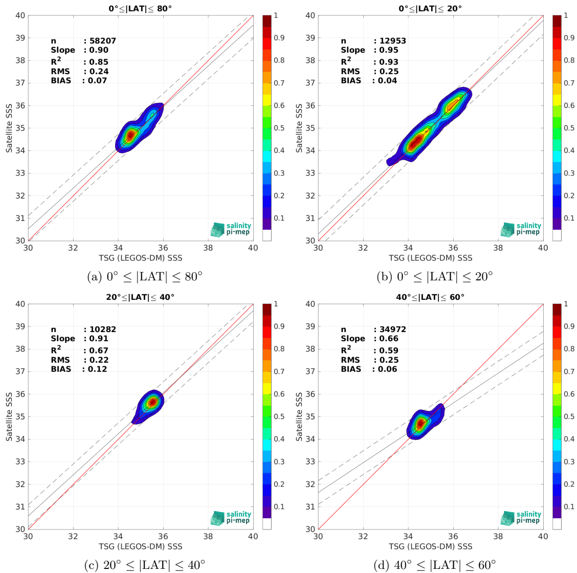
Figure 10: Contour maps of the concentration of Aquarius SSS L3 CAP v5 - Monthly (JPL) SSS (y-axis) versus TSG (LEGOS-DM) SSS (x-axis) at match-up pairs for different latitude bands. For each plot, the red line shows x=y . The black thin and dashed lines indicate a linear fit through the data cloud and the \pm 95\% confidence levels, respectively. The number match-up pairs n , the slope and R^2 coefficient of the linear fit, the root mean square (RMS) and the mean bias between satellite and in situ data are indicated for each latitude band in each plots.
