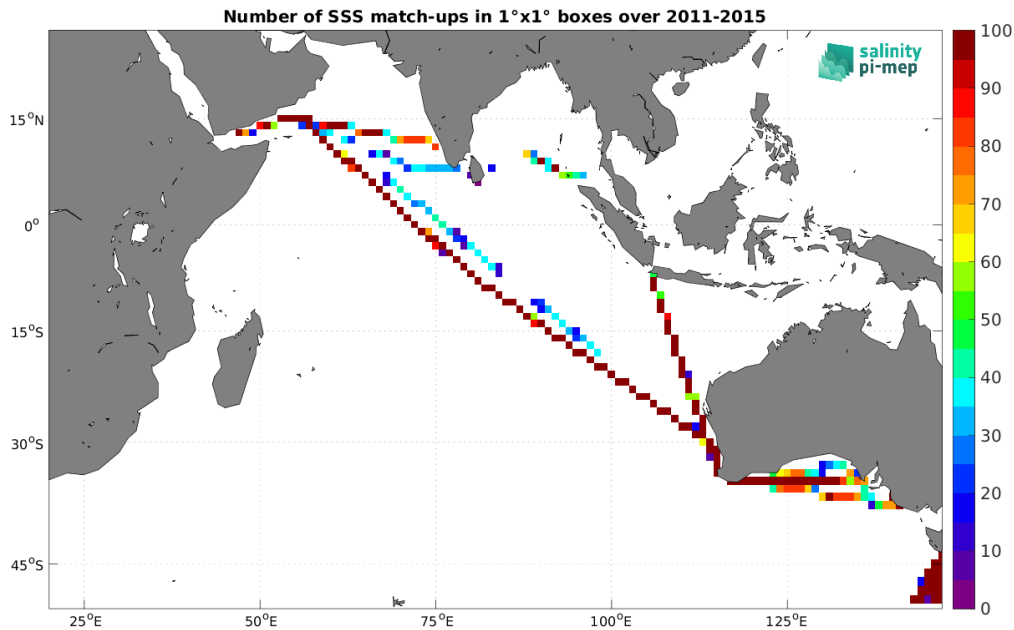
Figure 5: Number of SSS match-ups between TSG (LEGOS-DM) SSS and the Aquarius SSS L3 CAP v5 - Monthly (JPL) SSS product for the Indian Ocean Pi-MEP region over 1^\circ \times 1^\circ boxes and for the full satellite product period.
