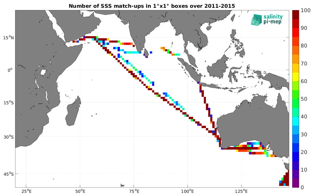
Figure 4: Number of SSS match-ups between TSG (LEGOS-DM) SSS and the Aquarius SSS L3 CAP v5 - Monthly (JPL) SSS product for the Indian Ocean Pi-MEP region over 1^\circ \times 1^\circ boxes and for the full satellite product period.
