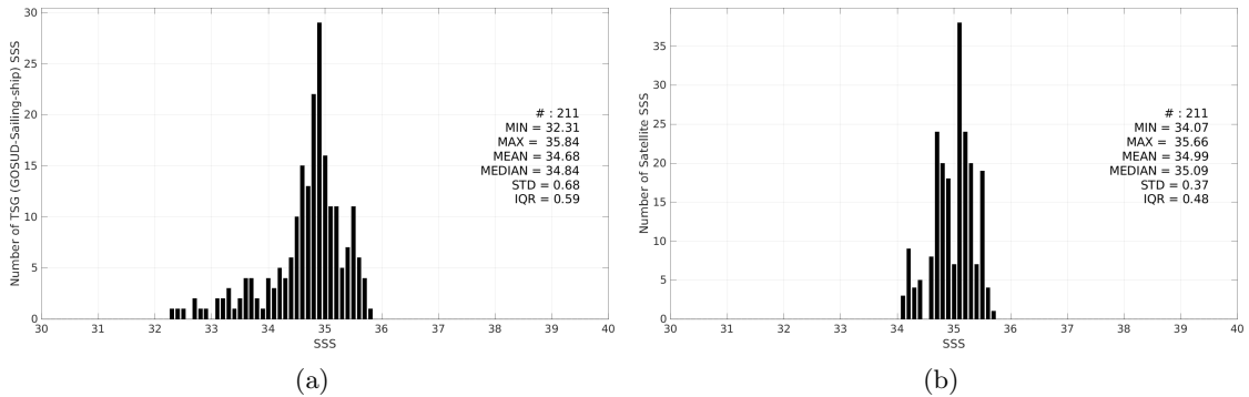
Figure 3: Histograms of SSS from TSG (GOSUD-Sailing-ship) (a) and Aquarius SSS L3 CAP v5 - Monthly (JPL) (b) considering all match-up pairs per bins of 0.1 over the Indian Ocean Pi-MEP region and for the full satellite product period.
