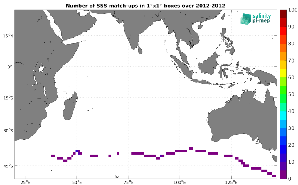
Figure 5: Number of SSS match-ups between TSG (GOSUD-Sailing-ship) SSS and the Aquarius SSS L3 CAP v5 - Monthly (JPL) SSS product for the Indian Ocean Pi-MEP region over 1^\circ \times 1^\circ boxes and for the full satellite product period.
