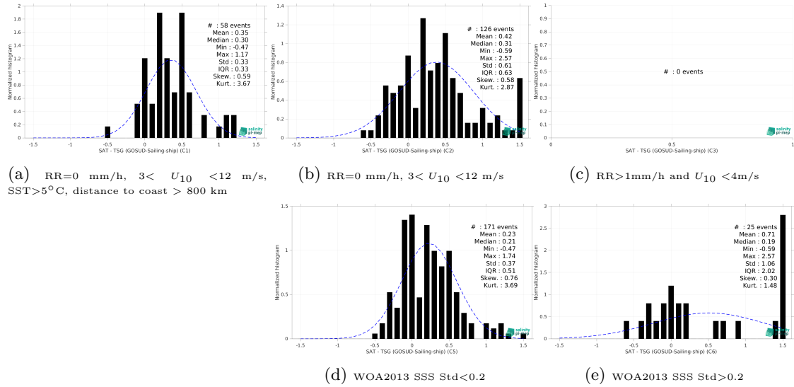
Figure 15: Normalized histogram of \Delta SSS (Aquarius SSS L3 CAP v5 - Monthly (JPL) - TSG (GOSUD-Sailing-ship)) for 5 different subdatasets corresponding to: RR=0 mm/h, 3 < U_{10} < 12 m/s, SST > 5°C, distance to coast > 800 km (a), RR=0 mm/h, 3 < U_{10} < 12 m/s (b), RR > 1mm/h and U_{10} < 4 m/s (c), WOA2013 SSS Std < 0.2 (d), WOA2013 SSS Std > 0.2 (e).
