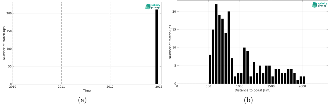
Figure 2: Number of match-ups between TSG (GOSUD-Sailing-ship) and Aquarius SSS L3 CAP v5 - Monthly (JPL) SSS as a function of time (a) and as function of the distance to coast (b) over the Indian Ocean Pi-MEP region and for the full satellite product period.
