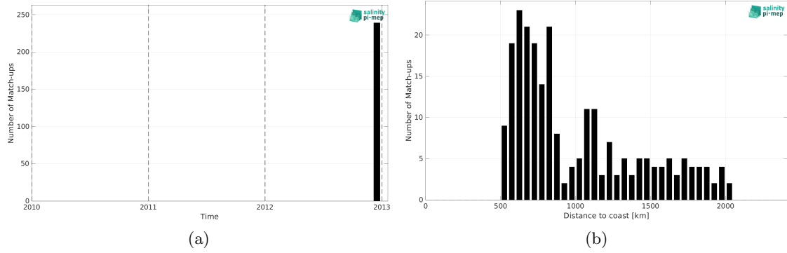
Figure 1: Number of match-ups between TSG (GOSUD-Sailing-ship) and Aquarius SSS L3 CAP v5 - Monthly (JPL) SSS as a function of time (a) and as function of the distance to coast (b) over the Indian Ocean Pi-MEP region and for the full satellite product period.
