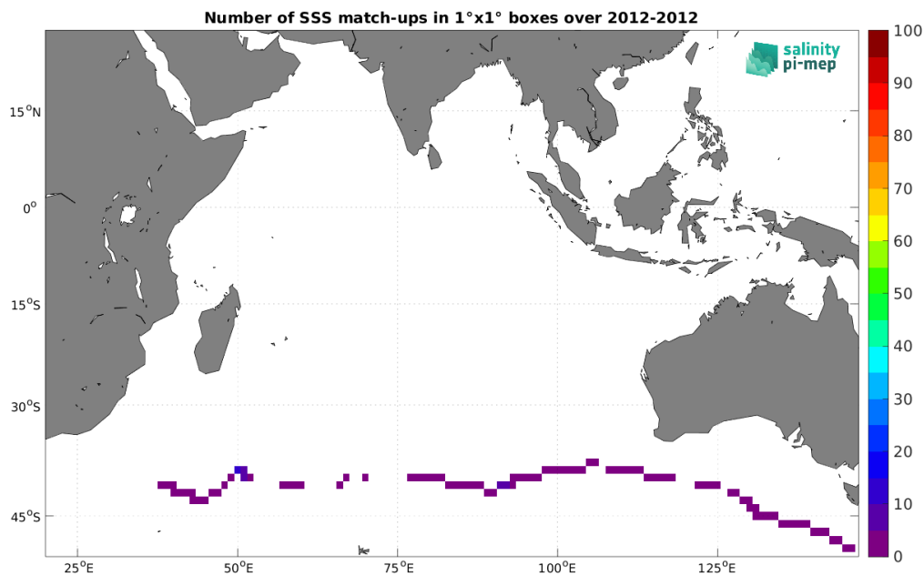
Figure 4: Number of SSS match-ups between TSG (GOSUD-Sailing-ship) SSS and the Aquarius SSS L3 CAP v5 - Monthly (JPL) SSS product for the Indian Ocean Pi-MEP region over 1^\circ \times 1^\circ boxes and for the full satellite product period.
