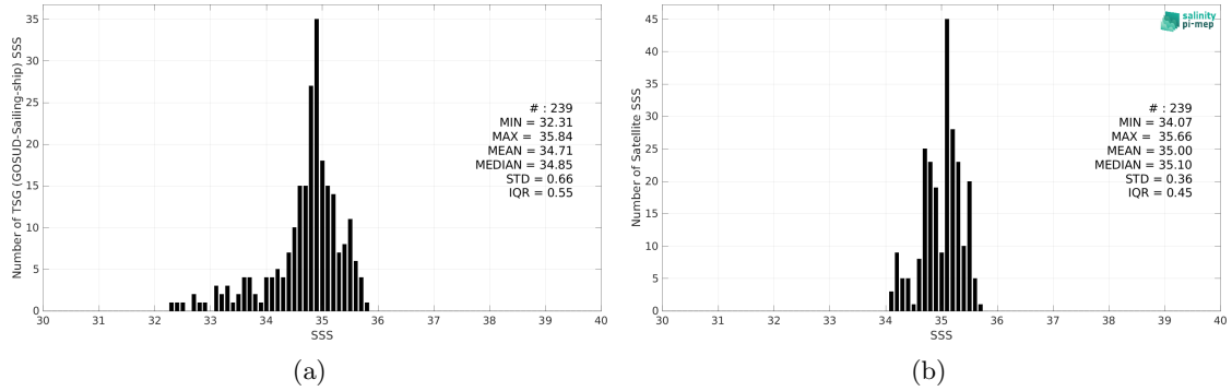
Figure 2: Histograms of SSS from TSG (GOSUD-Sailing-ship) (a) and Aquarius SSS L3 CAP v5 - Monthly (JPL) (b) considering all match-up pairs per bins of 0.1 over the Indian Ocean Pi-MEP region and for the full satellite product period.
