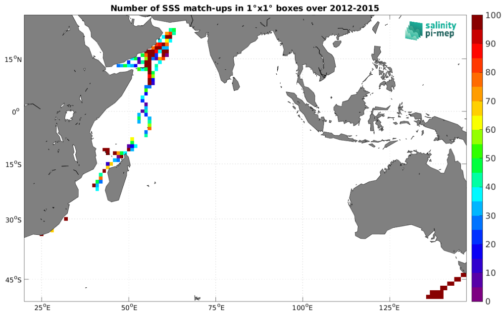
Figure 5: Number of SSS match-ups between TSG (GOSUD-Research-vessel) SSS and the Aquarius SSS L3 CAP v5 - Monthly (JPL) SSS product for the Indian Ocean Pi-MEP region over 1^\circ \times 1^\circ boxes and for the full satellite product period.
