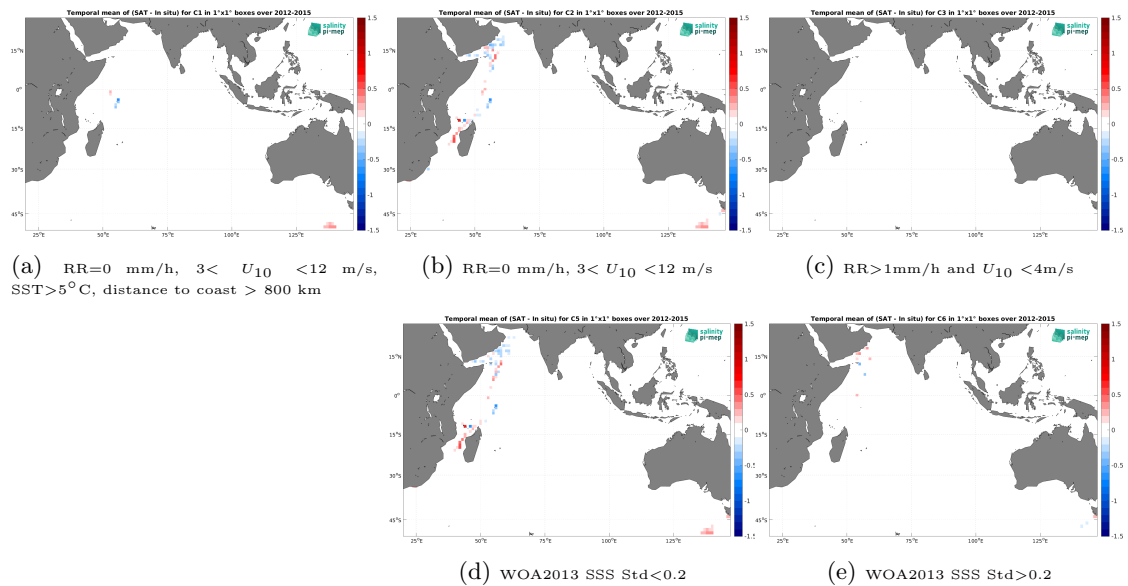
Figure 14: Temporal mean gridded over spatial boxes of size 1^\circ \times 1^\circ of \Delta\text{SSS} (Aquarius SSS L3 CAP v5 - Monthly (JPL) - TSG (GOSUD-Research-vessel)) for 5 different subdatasets corresponding to:RR=0 mm/h, 3 < U_{10} < 12 m/s, SST > 5°C, distance to coast > 800 km (a), RR=0 mm/h, 3 < U_{10} < 12 m/s (b), RR > 1mm/h and U_{10} < 4 m/s (c), WOA2013 SSS Std < 0.2 (d), WOA2013 SSS Std > 0.2 (e).
