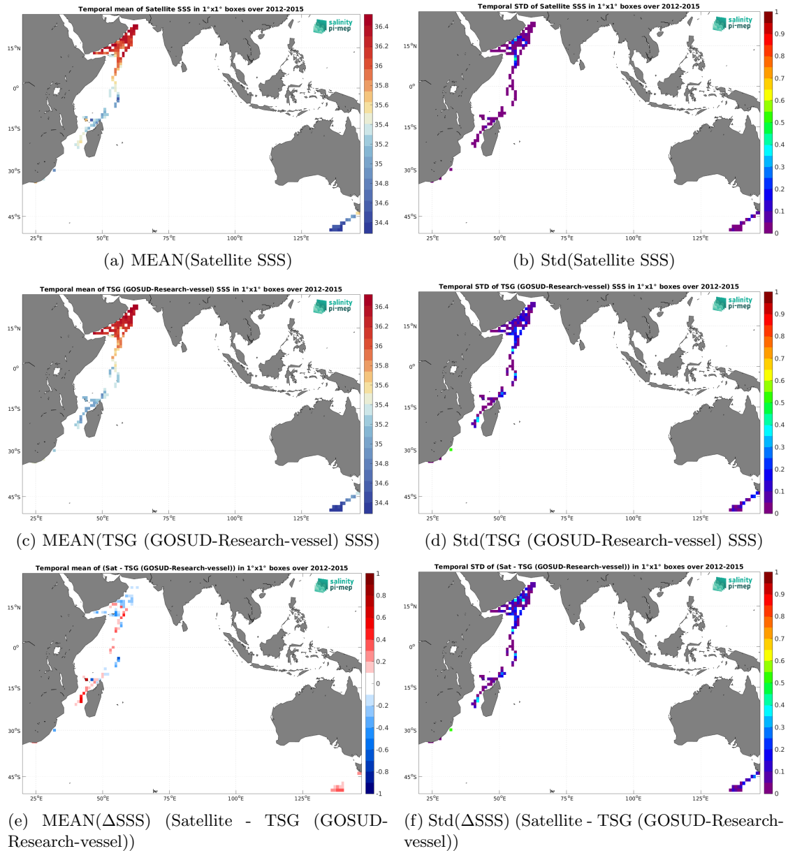
Figure 7: Temporal mean (left) and Std (right) of SSS from Aquarius SSS L3 CAP v5 - Monthly (JPL) (top), TSG (GOSUD-Research-vessel) (middle), and of \Delta SSS (Satellite - TSG (GOSUD-Research-vessel)). Only match-up pairs are used to generate these maps.
