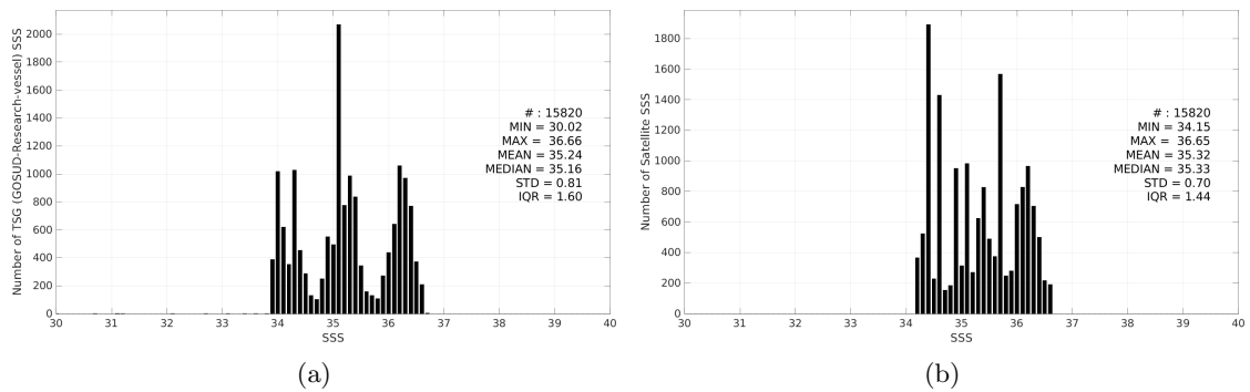
Figure 3: Histograms of SSS from TSG (GOSUD-Research-vessel) (a) and Aquarius SSS L3 CAP v5 - Monthly (JPL) (b) considering all match-up pairs per bins of 0.1 over the Indian Ocean Pi-MEP region and for the full satellite product period.
