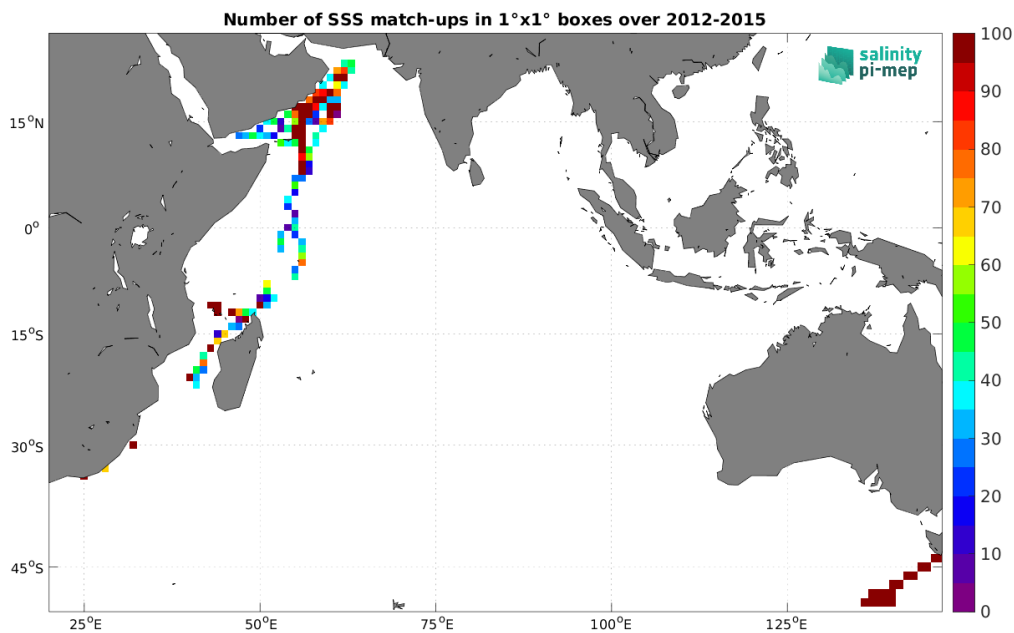
Figure 5: Number of SSS match-ups between TSG (GOSUD-Research-vessel) SSS and the Aquarius SSS L3 CAP v5 - Monthly (JPL) SSS product for the Indian Ocean Pi-MEP region over 1^\circ \times 1^\circ boxes and for the full satellite product period.
