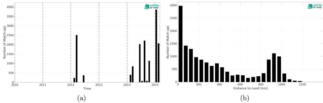
Figure 2: Number of match-ups between TSG (GOSUD-Research-vessel) and Aquarius SSS L3 CAP v5 - Monthly (JPL) SSS as a function of time (a) and as function of the distance to coast (b) over the Indian Ocean Pi-MEP region and for the full satellite product period.
