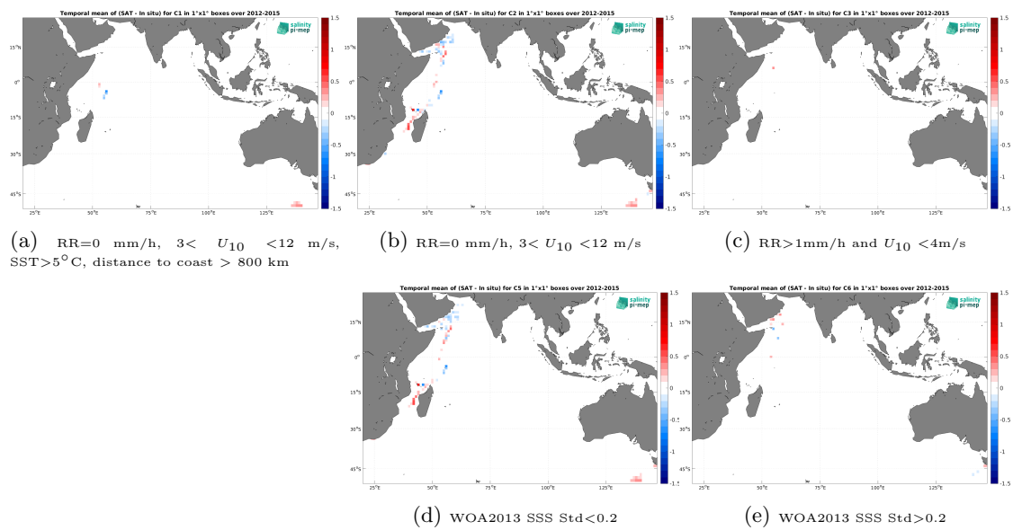
Figure 14: Temporal mean gridded over spatial boxes of size 1^\circ \times 1^\circ of \Delta SSS (Aquarius SSS L3 CAP v5 - Monthly (JPL) - TSG (GOSUD-Research-vessel)) for 5 different subdatasets corresponding to:RR=0 mm/h, 3 < U_{10} < 12 m/s, SST>5°C, distance to coast > 800 km (a), RR=0 mm/h, 3 < U_{10} < 12 m/s (b), RR>1mm/h and U_{10} < 4 m/s (c), WOA2013 SSS Std<0.2 (d), WOA2013 SSS Std>0.2 (e).
