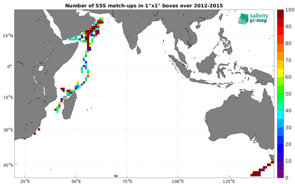
Figure 4: Number of SSS match-ups between TSG (GOSUD-Research-vessel) SSS and the Aquarius SSS L3 CAP v5 - Monthly (JPL) SSS product for the Indian Ocean Pi-MEP region over 1^\circ \times 1^\circ boxes and for the full satellite product period.
