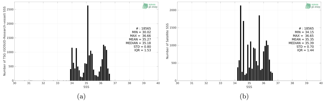
Figure 2: Histograms of SSS from TSG (GOSUD-Research-vessel) (a) and Aquarius SSS L3 CAP v5 - Monthly (JPL) (b) considering all match-up pairs per bins of 0.1 over the Indian Ocean Pi-MEP region and for the full satellite product period.
