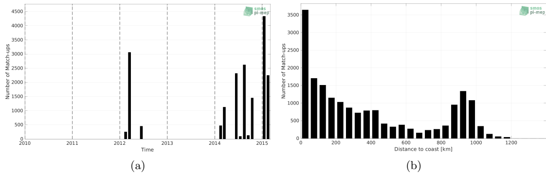
Figure 1: Number of match-ups between TSG (GOSUD-Research-vessel) and Aquarius SSS L3 CAP v5 - Monthly (JPL) SSS as a function of time (a) and as function of the distance to coast (b) over the Indian Ocean Pi-MEP region and for the full satellite product period.
