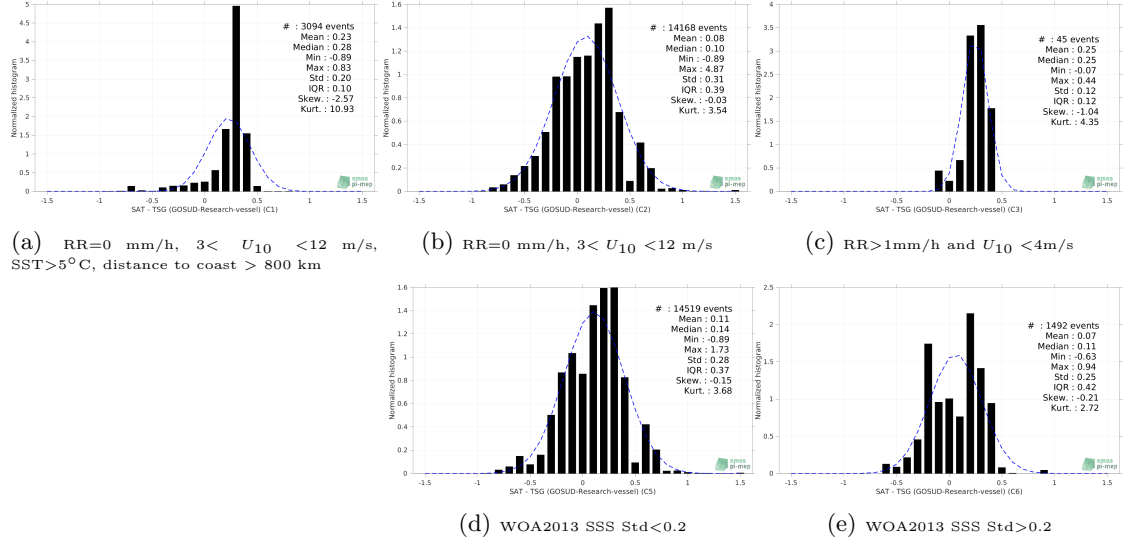
Figure 13: Normalized histogram of \Delta\text{SSS} (Aquarius SSS L3 CAP v5 - Monthly (JPL) - TSG (GOSUD-Research-vessel)) for 5 different subdatasets corresponding to: RR=0 mm/h, 3 < U_{10} < 12 m/s, SST > 5^\circ\text{C} , distance to coast > 800 km (a), RR=0 mm/h, 3 < U_{10} < 12 m/s (b), RR > 1 mm/h and U_{10} < 4 m/s (c), WOA2013 SSS Std < 0.2 (d), WOA2013 SSS Std > 0.2 (e).
