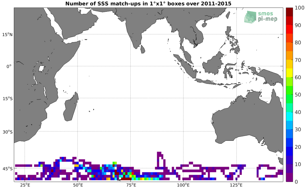
Figure 4: Number of SSS match-ups between Sea mammals SSS and the Aquarius SSS L3 CAP v5 - Monthly (JPL) SSS product for the Indian Ocean Pi-MEP region over 1^\circ \times 1^\circ boxes and for the full satellite product period.
