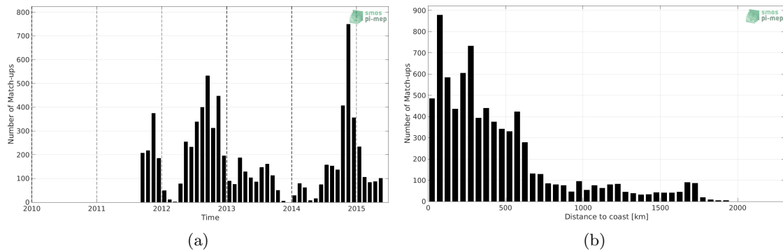
Figure 1: Number of match-ups between Sea mammals and Aquarius SSS L3 CAP v5 - Monthly (JPL) SSS as a function of time (a) and as function of the distance to coast (b) over the Indian Ocean Pi-MEP region and for the full satellite period.
