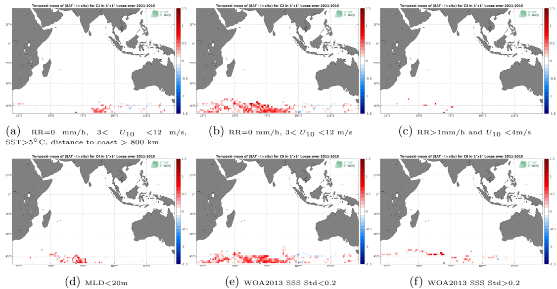
Figure 12: Temporal mean gridded over spatial boxes of size 1^{\circ}\times 1^{\circ} of \Delta\text{SSS} (Aquarius SSS L3 CAP v5 - Monthly (JPL) - Sea mammals) for 6 different subdatasets corresponding to:RR=0 mm/h, 3 < U_{10} < 12 m/s, SST > 5^{\circ}\text{C} , distance to coast > 800 km (a), RR=0 mm/h, 3 < U_{10} < 12 m/s (b), RR > 1\text{mm/h} and U_{10} < 4\text{m/s} (c),MLD < 20\text{m} (d),WOA2013 SSS Std < 0.2 (e),WOA2013 SSS Std > 0.2 (f).
