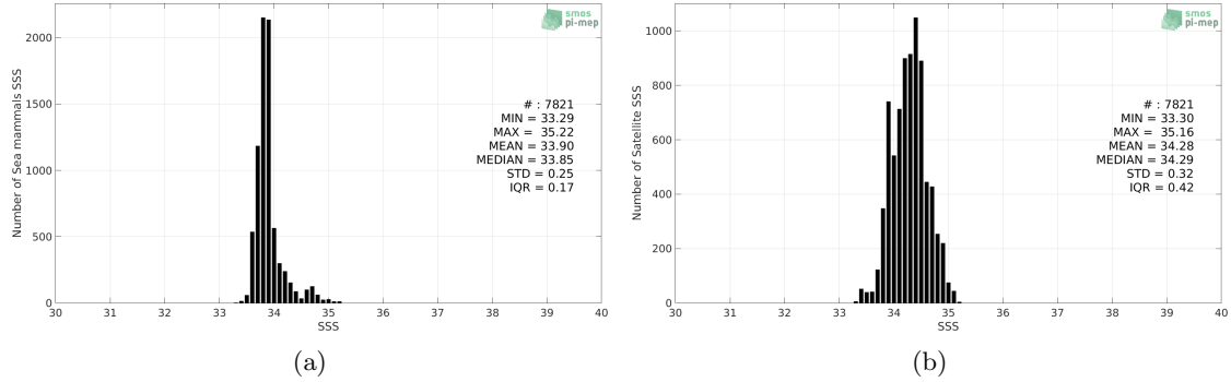
Figure 2: Histograms of SSS from Sea mammals (a) and Aquarius SSS L3 CAP v5 - Monthly (JPL) (b) considering all match-up pairs per bins of 0.1 over the Indian Ocean Pi-MEP region and for the full satellite product period.
