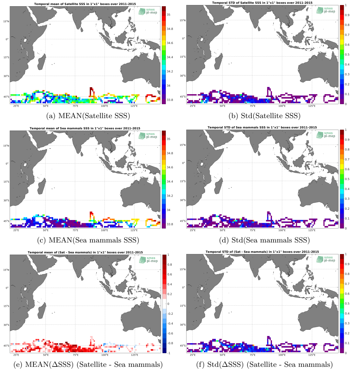
Figure 6: Temporal mean (left) and Std (right) of SSS from Aquarius SSS L3 CAP v5 - Monthly (JPL) (top), Sea mammals (middle), and of \Delta SSS (Satellite - Sea mammals). Only match-up pairs are used to generate these maps.
