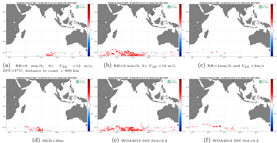
Figure 12: Temporal mean gridded over spatial boxes of size 1^{\circ}\times 1^{\circ} of \Delta\text{SSS} (Aquarius-L3-JPL-V5-MONTHLY - Sea mammals) for 6 different subdatasets corresponding to:RR=0 mm/h, 3 < U_{10} < 12 m/s, SST > 5^{\circ}\text{C} , distance to coast > 800 km (a), RR=0 mm/h, 3 < U_{10} < 12 m/s (b), RR > 1\text{mm/h} and U_{10} < 4\text{m/s} (c),MLD < 20\text{m} (d),WOA2013 SSS Std < 0.2 (e),WOA2013 SSS Std > 0.2 (f).
