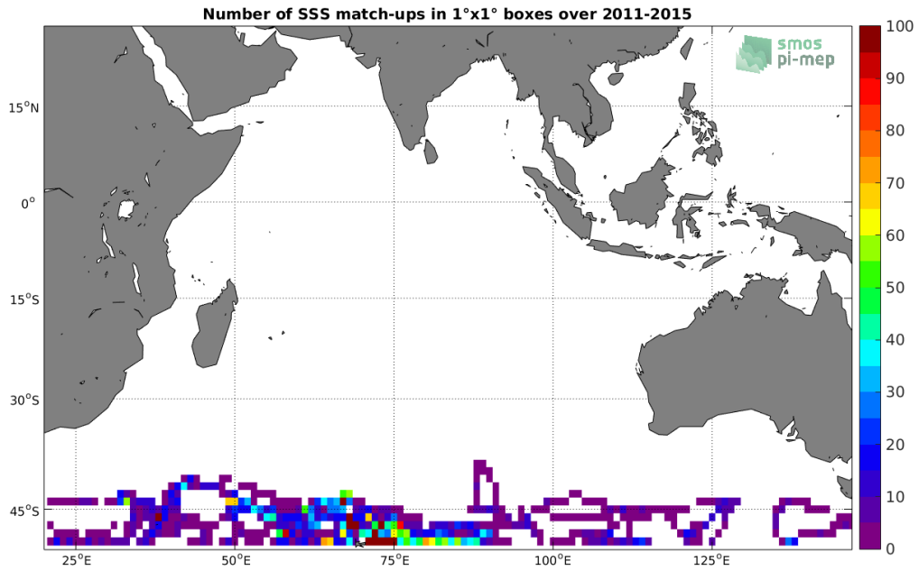
Figure 4: Number of SSS match-ups between Sea mammals SSS and the Aquarius-L3-JPL-V5-MONTHLY SSS product for the Indian Ocean Pi-MEP region over 1^\circ \times 1^\circ boxes and for the full satellite product period.
