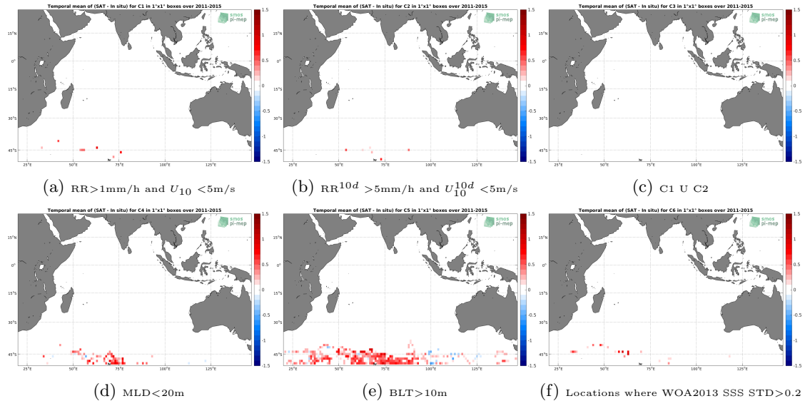
Figure 12: Temporal mean gridded over spatial boxes of size 1^\circ \times 1^\circ of \Delta\text{SSS} (Aquarius-L3-JPL-V5-MONTHLY - Sea mammals) for 6 different subdatasets corresponding to: RR > 1\text{mm/h} and U_{10} < 5\text{m/s} (a), RR^{10d} > 5\text{mm/h} and U_{10}^{10d} < 5\text{m/s} (b), C1 U C2 (c), MLD < 20\text{m} (d), BLT > 10\text{m} (e), Locations where WOA2013 SSS STD > 0.2 (f).
