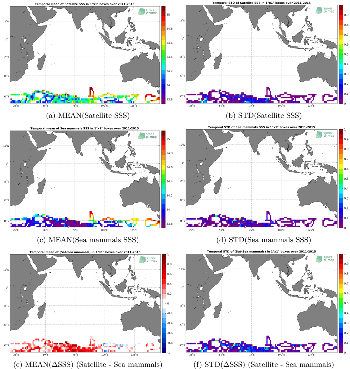
Figure 6: Temporal mean (left) and STD (right) of SSS from Aquarius-L3-JPL-V5-MONTHLY (top), Sea mammals (middle), and of \Delta SSS (Satellite - Sea mammals). Only match-up pairs are used to generate these maps.
