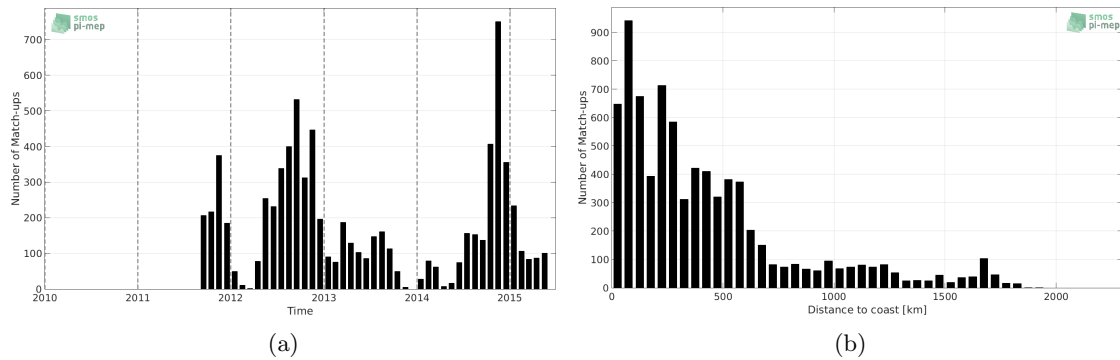
Figure 1: Number of match-ups between Sea mammals and Aquarius-L3-JPL-V5-MONTHLY SSS as a function of time (a) and as function of the distance to coast (b) over the Indian Ocean Pi-MEP region and for the full satellite product period.
