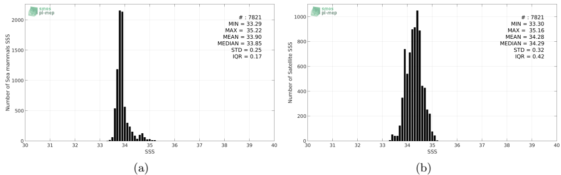
Figure 2: Histograms of SSS from Sea mammals (a) and Aquarius-L3-JPL-V5-MONTHLY (b) considering all match-up pairs per bins of 0.1 over the Indian Ocean Pi-MEP region and for the full satellite product period.
