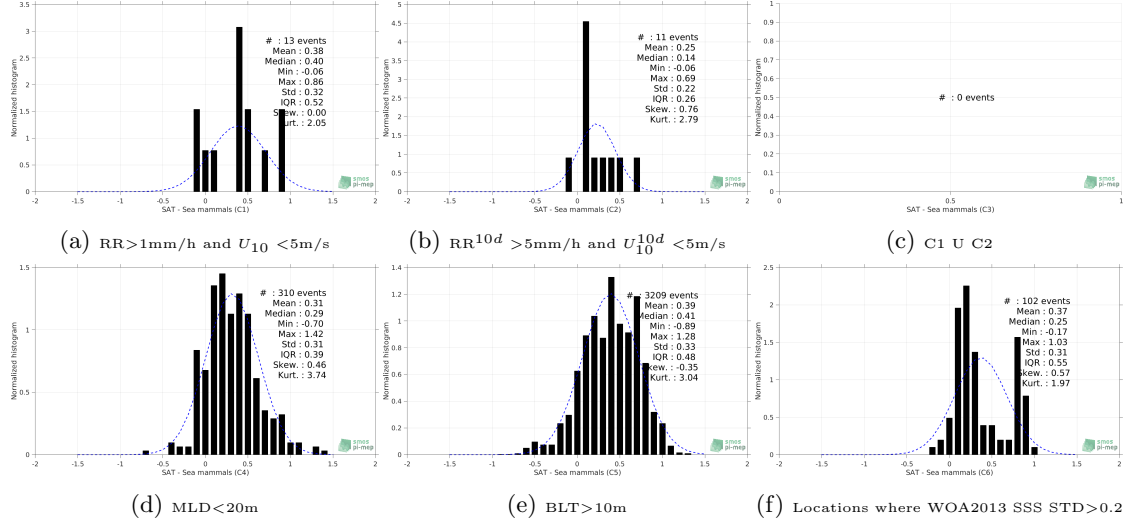
Figure 13: Normalized histogram of \Delta SSS (Aquarius-L3-JPL-V5-MONTHLY - Sea mammals) for 6 different subdatasets corresponding to: RR > 1\text{mm/h} and U_{10} < 5\text{m/s} (a), RR^{10d} > 5\text{mm/h} and U_{10}^{10d} < 5\text{m/s} (b), C1 \cup C2 (c), MLD < 20\text{m} (d), BLT > 10\text{m} (e), Locations where WOA2013 SSS STD > 0.2 (f).
