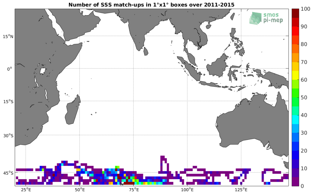
Figure 4: Number of SSS match-ups between Sea mammals SSS and the Aquarius-L3-JPL-V5-MONTHLY SSS product for the Indian Ocean Pi-MEP region over 1°x1° boxes and for the full satellite product period.
