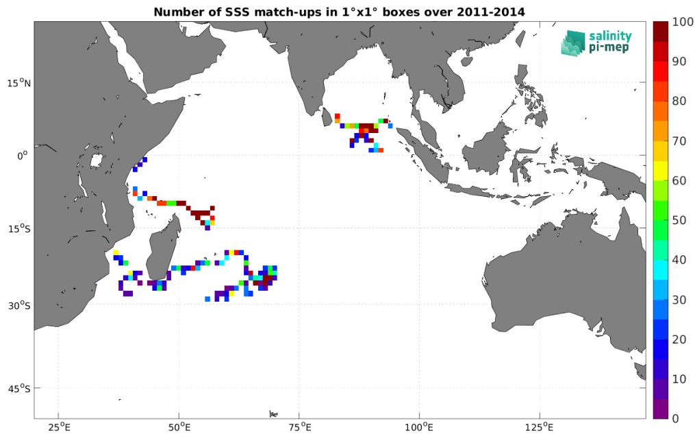
Figure 4: Number of SSS match-ups between Surface drifters SSS and the Aquarius SSS L3 CAP v5 - Monthly (JPL) SSS product for the Indian Ocean Pi-MEP region over 1^\circ \times 1^\circ boxes and for the full satellite product period.
