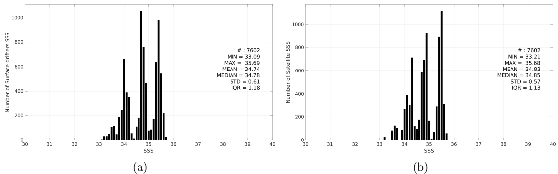
Figure 3: Histograms of SSS from Surface drifters (a) and Aquarius SSS L3 CAP v5 - Monthly (JPL) (b) considering all match-up pairs per bins of 0.1 over the Indian Ocean Pi-MEP region and for the full satellite product period.
