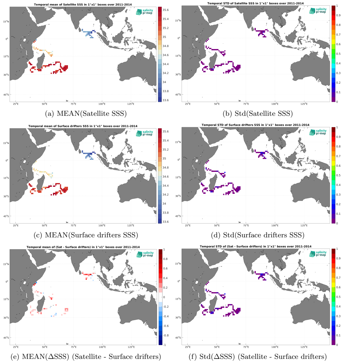
Figure 6: Temporal mean (left) and Std (right) of SSS from Aquarius SSS L3 CAP v5 - Monthly (JPL) (top), Surface drifters (middle), and of \Delta SSS (Satellite - Surface drifters). Only match-up pairs are used to generate these maps.
