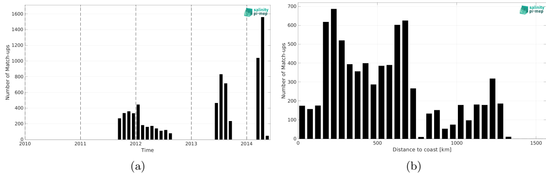
Figure 2: Number of match-ups between Surface drifters and Aquarius SSS L3 CAP v5 - Monthly (JPL) SSS as a function of time (a) and as function of the distance to coast (b) over the Indian Ocean Pi-MEP region and for the full satellite product period.
