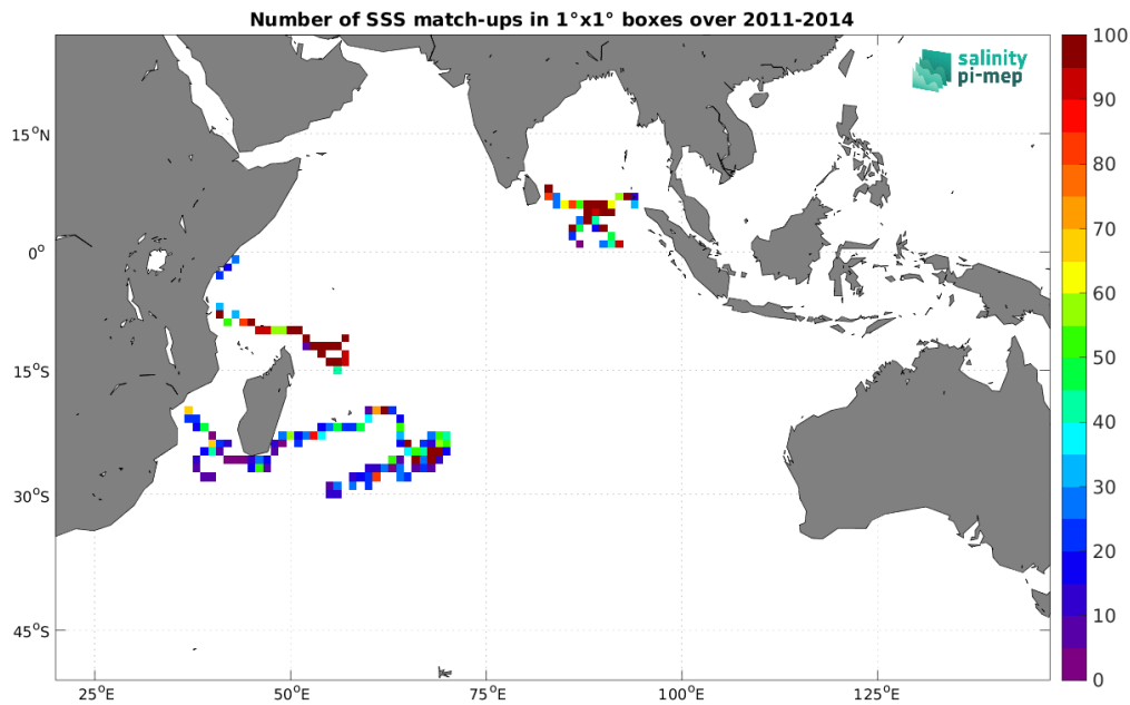
Figure 3: Number of SSS match-ups between Surface drifters SSS and the Aquarius SSS L3 CAP v5 - Monthly (JPL) SSS product for the Indian Ocean Pi-MEP region over 1^\circ \times 1^\circ boxes and for the full satellite product period.
