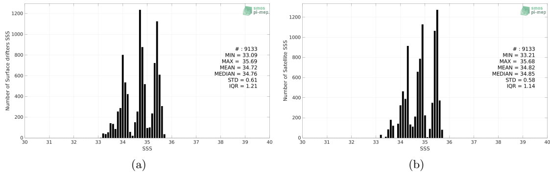
Figure 2: Histograms of SSS from Surface drifters (a) and Aquarius SSS L3 CAP v5 - Monthly (JPL) (b) considering all match-up pairs per bins of 0.1 over the Indian Ocean Pi-MEP region and for the full satellite product period.
