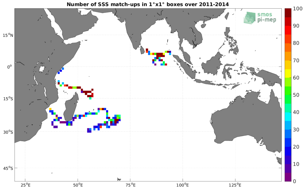
Figure 3: Number of SSS match-ups between Surface drifters SSS and the Aquarius SSS L3 CAP v5 - Monthly (JPL) SSS product for the Indian Ocean Pi-MEP region over 1^\circ \times 1^\circ boxes and for the full satellite product period.
