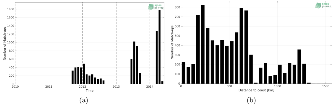
Figure 1: Number of match-ups between Surface drifters and Aquarius SSS L3 CAP v5 - Monthly (JPL) SSS as a function of time (a) and as function of the distance to coast (b) over the Indian Ocean Pi-MEP region and for the full satellite product period.
