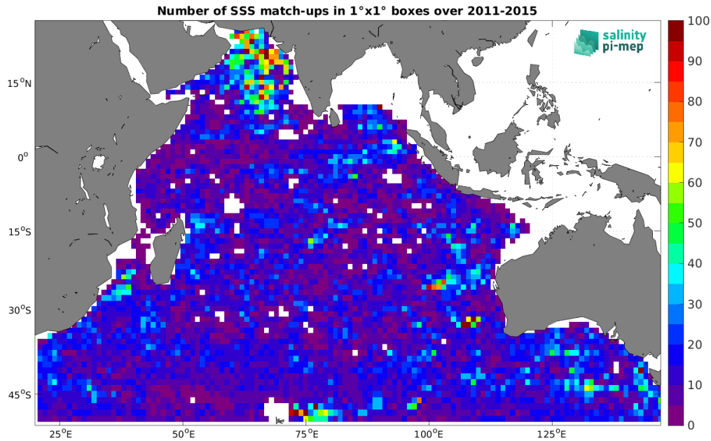
Figure 4: Number of SSS match-ups between Argo SSS and the Aquarius SSS L3 CAP v5 - Monthly (JPL) SSS product for the Indian Ocean Pi-MEP region over 1^\circ \times 1^\circ boxes and for the full satellite product period.
