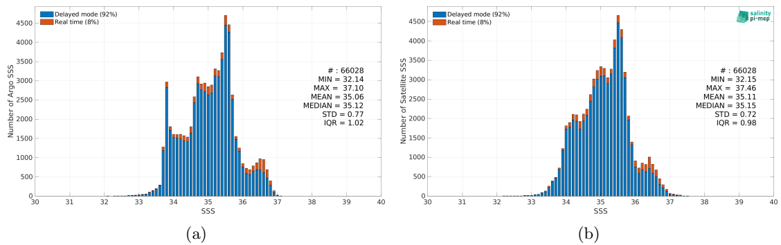
Figure 2: Histograms of SSS from Argo (a) and Aquarius SSS L3 CAP v5 - Monthly (JPL) (b) considering all match-up pairs per bins of 0.1 over the Indian Ocean Pi-MEP region and for the full satellite product period.
