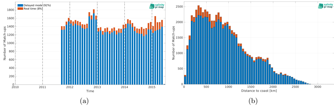
Figure 1: Number of match-ups between Argo and Aquarius SSS L3 CAP v5 - Monthly (JPL) SSS as a function of time (a) and as function of the distance to coast (b) over the Indian Ocean Pi-MEP region and for the full satellite product period.
