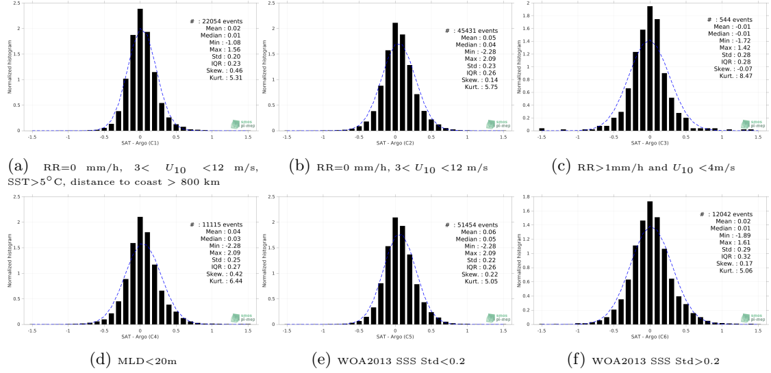
Figure 13: Normalized histogram of \Delta SSS (Aquarius SSS L3 CAP v5 - Monthly (JPL) - Argo) for 6 different subdatasets corresponding to: RR=0 mm/h, 3 < U_{10} < 12 m/s, SST>5°C, distance to coast > 800 km (a), RR=0 mm/h, 3 < U_{10} < 12 m/s (b), RR>1mm/h and U_{10} < 4 m/s (c), MLD<20m (d), WOA2013 SSS Std<0.2 (e), WOA2013 SSS Std>0.2 (f).
