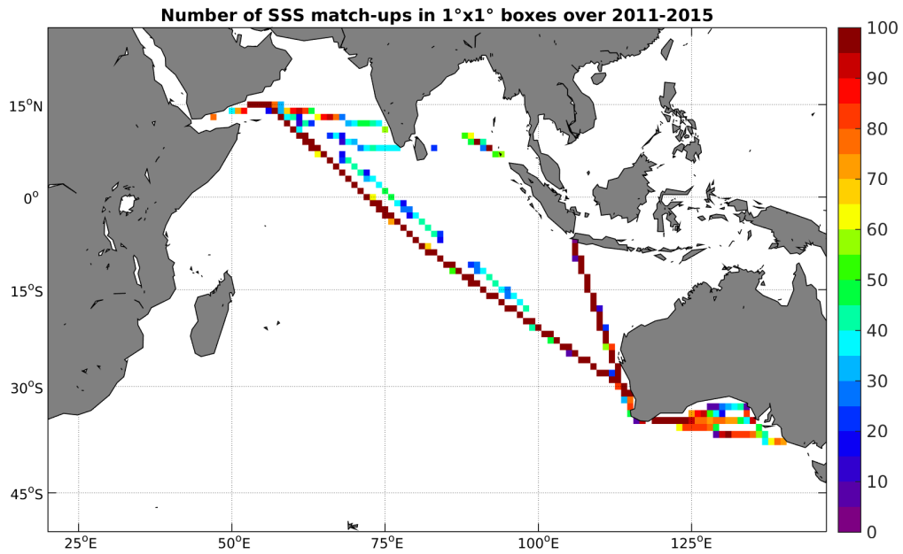
Figure 4: Number of SSS match-ups between TSG-LEGOS-DM SSS and the Aquarius-L3-JPL-V4-7DAY-RUNNING SSS product for the Indian Ocean Pi-MEP region over 1°x1° boxes and for the full satellite product period.
