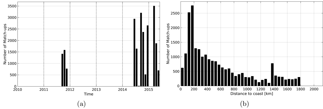
Figure 1: Number of match-ups between TSG-LEGOS-DM and Aquarius-L3-JPL-V4-7DAY-RUNNING SSS as a function of time (a) and as function of the distance to coast (b) over the Indian Ocean Pi-MEP region and for the full satellite product period.
