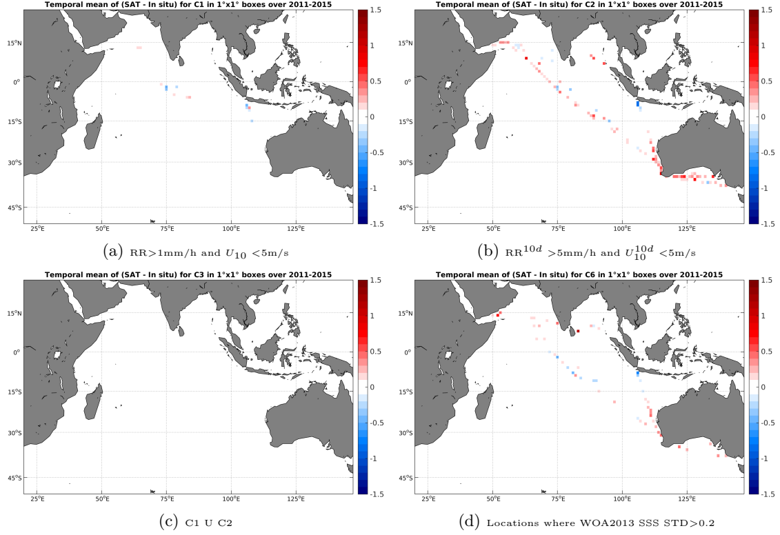
Figure 12: Temporal mean gridded over spatial boxes of size 1^\circ \times 1^\circ of \Delta SSS (Aquarius-L3-JPL-V4-7DAY-RUNNING - TSG-LEGOS-DM) for 4 different subdatasets corresponding to: RR > 1 mm/h and U_{10} < 5 m/s (a), RR^{10d} > 5 mm/h and U_{10}^{10d} < 5 m/s (b), C1 U C2 (c), Locations where WOA2013 SSS STD > 0.2 (d).
