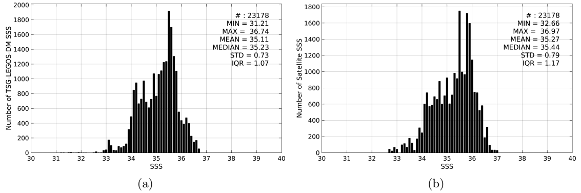
Figure 2: Histograms of SSS from TSG-LEGOS-DM (a) and Aquarius-L3-JPL-V4-7DAY-RUNNING (b) considering all match-up pairs per bins of 0.1 over the Indian Ocean Pi-MEP region and for the full satellite product period.
