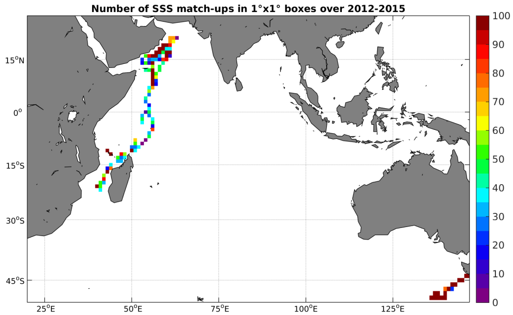
Figure 4: Number of SSS match-ups between TSG-GOSUD-Research-vessel SSS and the Aquarius-L3-JPL-V4-7DAY-RUNNING SSS product for the Indian Ocean Pi-MEP region over 1^\circ \times 1^\circ boxes and for the full satellite product period.
