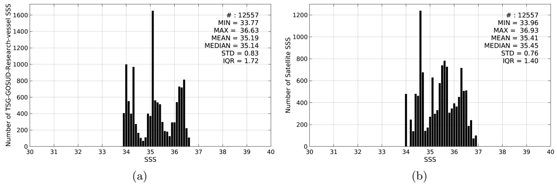
Figure 2: Histograms of SSS from TSG-GOSUD-Research-vessel (a) and Aquarius-L3-JPL-V4-7DAY-RUNNING (b) considering all match-up pairs per bins of 0.1 over the Indian Ocean Pi-MEP region and for the full satellite product period.
