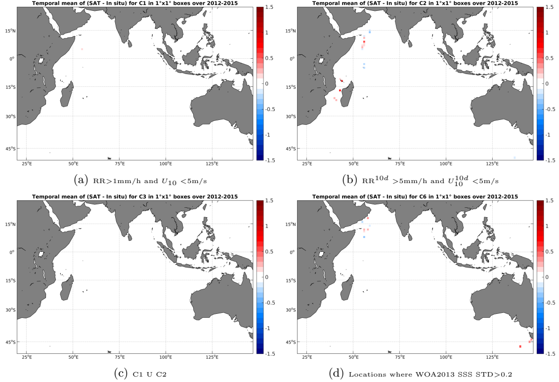
Figure 12: Temporal mean gridded over spatial boxes of size 1^\circ \times 1^\circ of \Delta SSS (Aquarius-L3-JPL-V4-7DAY-RUNNING - TSG-GOSUD-Research-vessel) for 4 different subdatasets corresponding to: RR > 1mm/h and U_{10} < 5 m/s (a), RR^{10d} > 5 mm/h and U_{10}^{10d} < 5 m/s (b), C1 U C2 (c), Locations where WOA2013 SSS STD > 0.2 (d).
