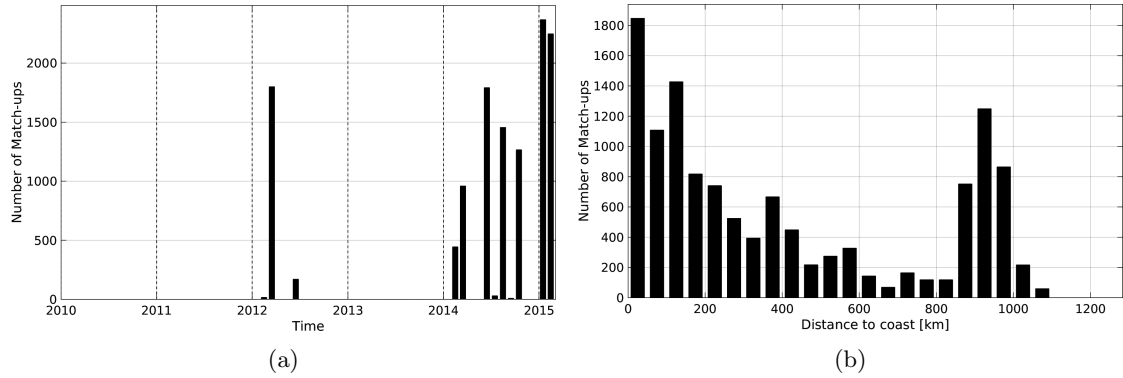
Figure 1: Number of match-ups between TSG-GOSUD-Research-vessel and Aquarius-L3-JPL-V4-7DAY-RUNNING SSS as a function of time (a) and as function of the distance to coast (b) over the Indian Ocean Pi-MEP region and for the full satellite product period.
