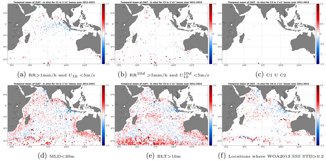
Figure 12: Temporal mean gridded over spatial boxes of size 1^\circ \times 1^\circ of \Delta SSS (Aquarius-L3-JPL-V4-7DAY-RUNNING - Argo) for 6 different subdatasets corresponding to: RR > 1\text{mm/h} and U_{10} < 5\text{m/s} (a), RR^{10d} > 5\text{mm/h} and U_{10}^{10d} < 5\text{m/s} (b), C1 U C2 (c), MLD < 20\text{m} (d), BLT > 10\text{m} (e), Locations where WOA2013 SSS STD > 0.2 (f).
