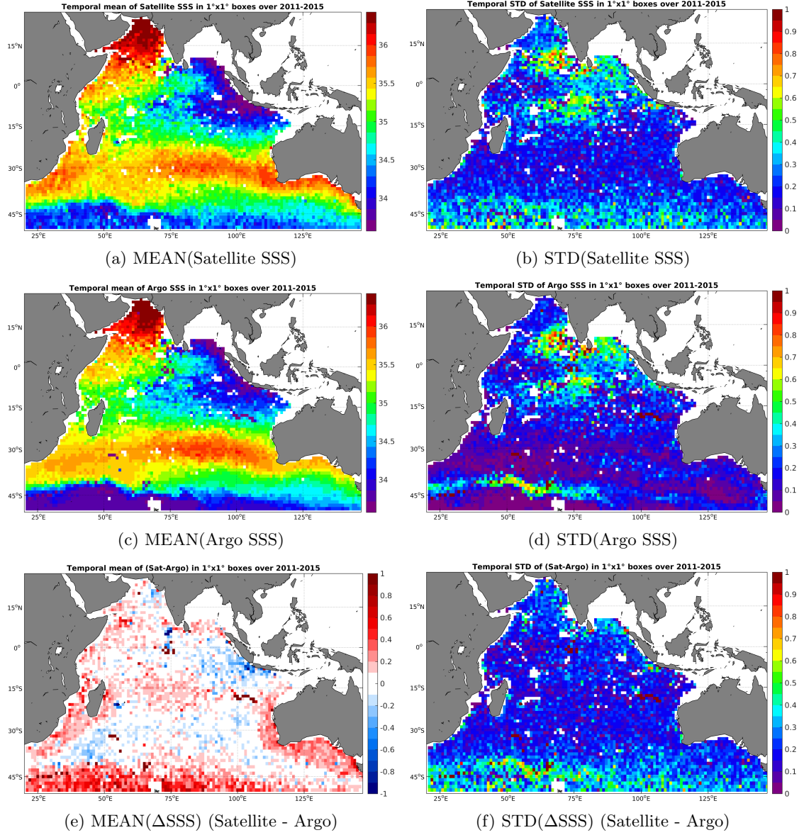
Figure 6: Temporal mean (left) and STD (right) of SSS from Aquarius-L3-JPL-V4-7DAY-RUNNING (top), Argo (middle), and of \Delta SSS (Satellite - Argo). Only match-up pairs are used to generate these maps.
