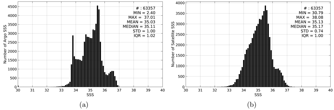
Figure 2: Histograms of SSS from Argo (a) and Aquarius-L3-JPL-V4-7DAY-RUNNING (b) considering all match-up pairs per bins of 0.1 over the Indian Ocean Pi-MEP region and for the full satellite product period.
