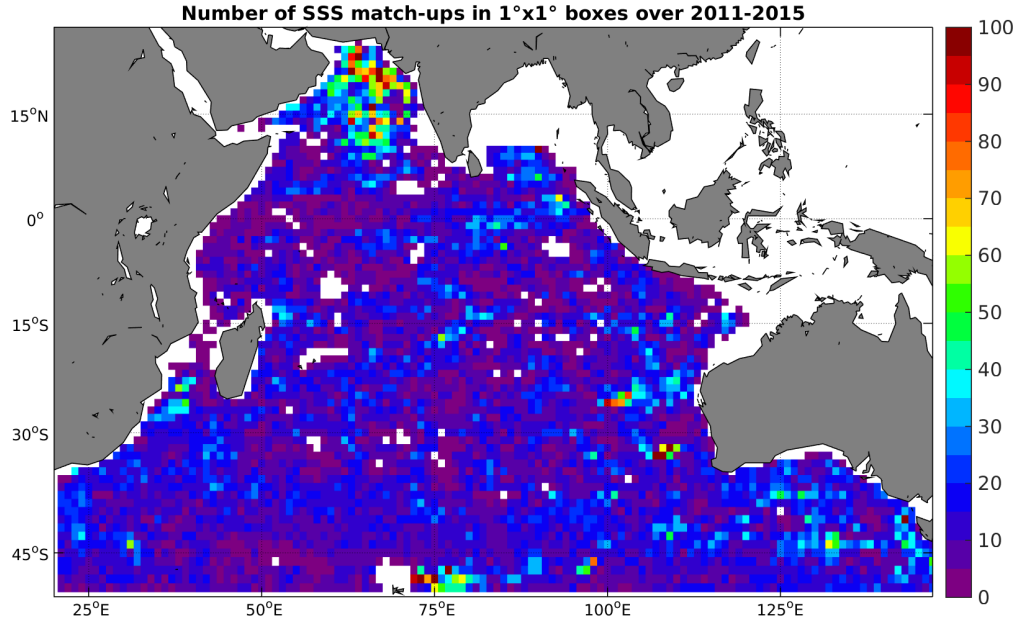
Figure 4: Number of SSS match-ups between Argo SSS and the Aquarius-L3-JPL-V4-7DAY-RUNNING SSS product for the Indian Ocean Pi-MEP region over 1^\circ \times 1^\circ boxes and for the full satellite product period.
