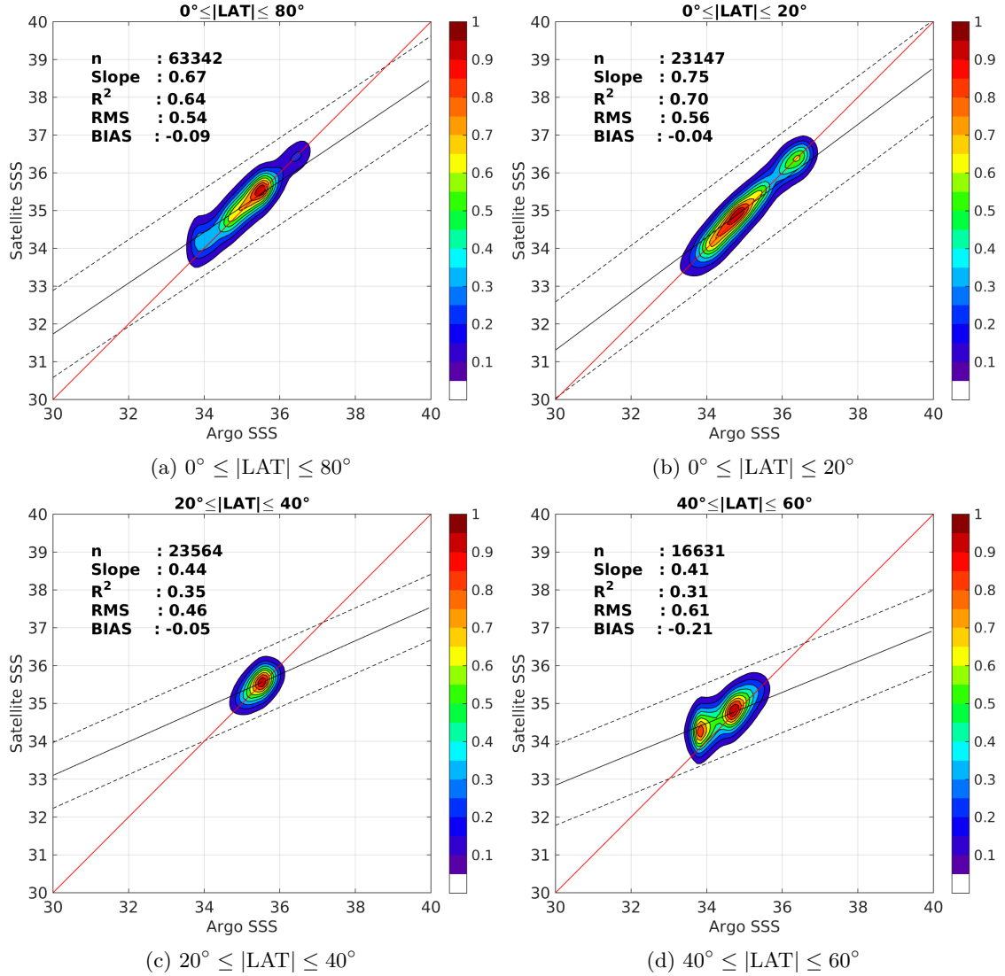
Figure 9: Contour maps of the concentration of Aquarius-L3-JPL-V4-7DAY-RUNNING SSS (y-axis) versus Argo SSS (x-axis) at match-up pairs for different latitude bands. For each plot, the red line shows x=y . The black thin and dashed lines indicate a linear fit through the data cloud and the \pm 95\% confidence levels, respectively. The number match-up pairs n , the slope and R^2 coefficient of the linear fit, the root mean square (RMS) and the mean bias between satellite and in situ data are indicated for each latitude band in each plots.
