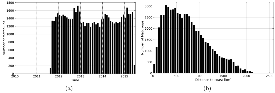
Figure 1: Number of match-ups between Argo and Aquarius-L3-JPL-V4-7DAY-RUNNING SSS as a function of time (a) and as function of the distance to coast (b) over the Indian Ocean Pi-MEP region and for the full satellite product period.
