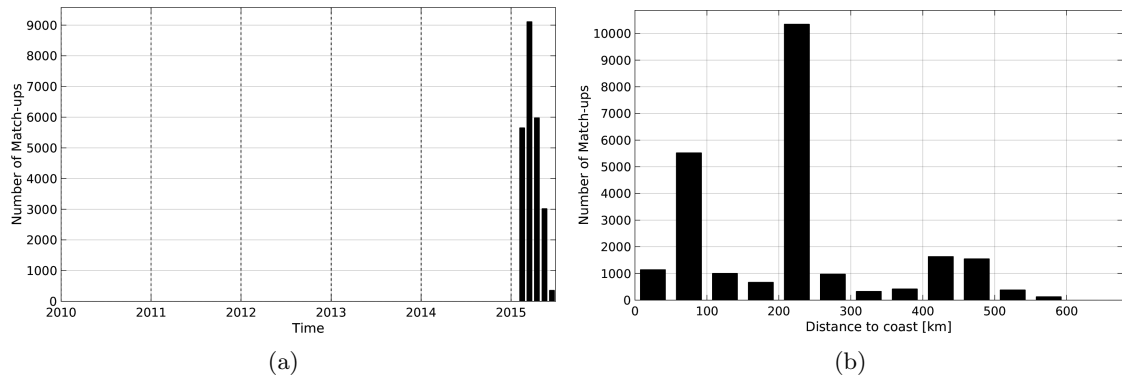
Figure 1: Number of match-ups between TSG-SAMOS and Aquarius-L3-JPL-V4-MONTHLY SSS as a function of time (a) and as function of the distance to coast (b) over the Indian Ocean Pi-MEP region and for the full satellite product period.
