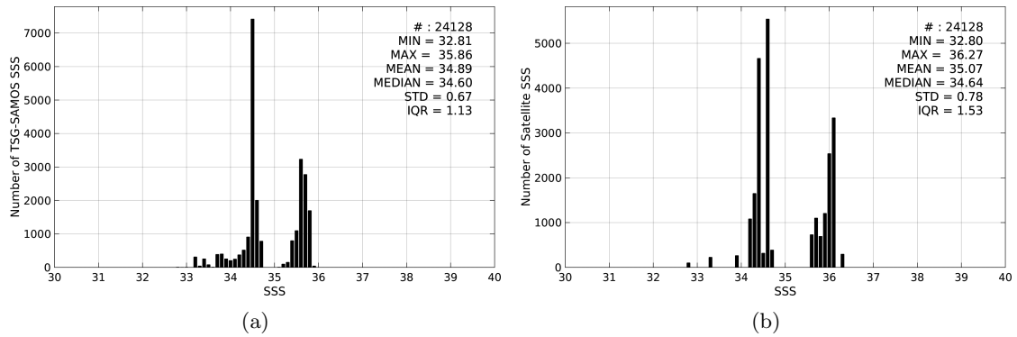
Figure 2: Histograms of SSS from TSG-SAMOS (a) and Aquarius-L3-JPL-V4-MONTHLY (b) considering all match-up pairs per bins of 0.1 over the Indian Ocean Pi-MEP region and for the full satellite product period.
