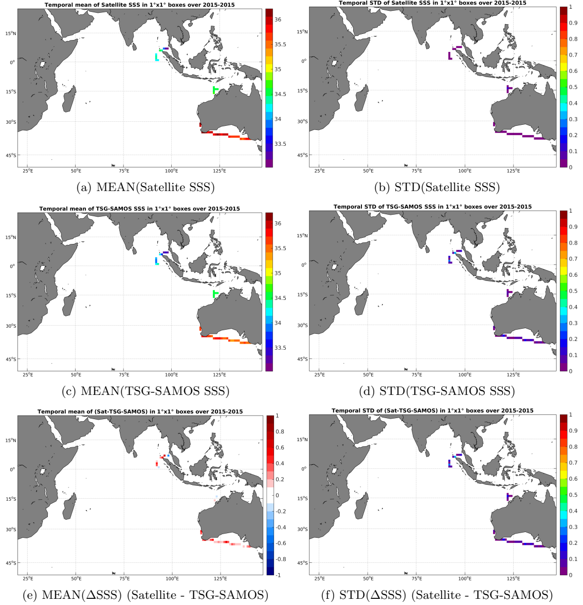
Figure 6: Temporal mean (left) and STD (right) of SSS from Aquarius-L3-JPL-V4-MONTHLY (top), TSG-SAMOS (middle), and of \Delta SSS (Satellite - TSG-SAMOS). Only match-up pairs are used to generate these maps.
