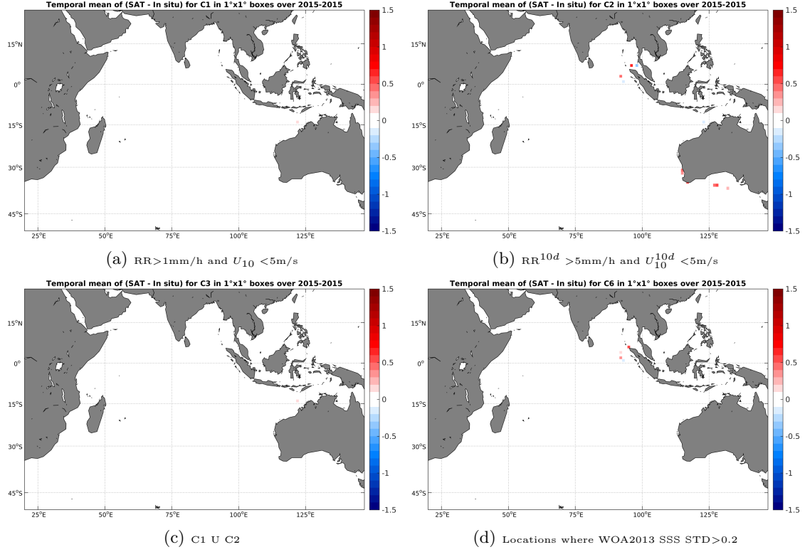
Figure 12: Temporal mean gridded over spatial boxes of size 1^\circ \times 1^\circ of \Delta SSS (Aquarius-L3-JPL-V4-MONTHLY - TSG-SAMOS) for 4 different subdatasets corresponding to: RR > 1 mm/h and U_{10} < 5 m/s (a), RR^{10d} > 5 mm/h and U_{10}^{10d} < 5 m/s (b), C1 U C2 (c), Locations where WOA2013 SSS STD > 0.2 (d).
