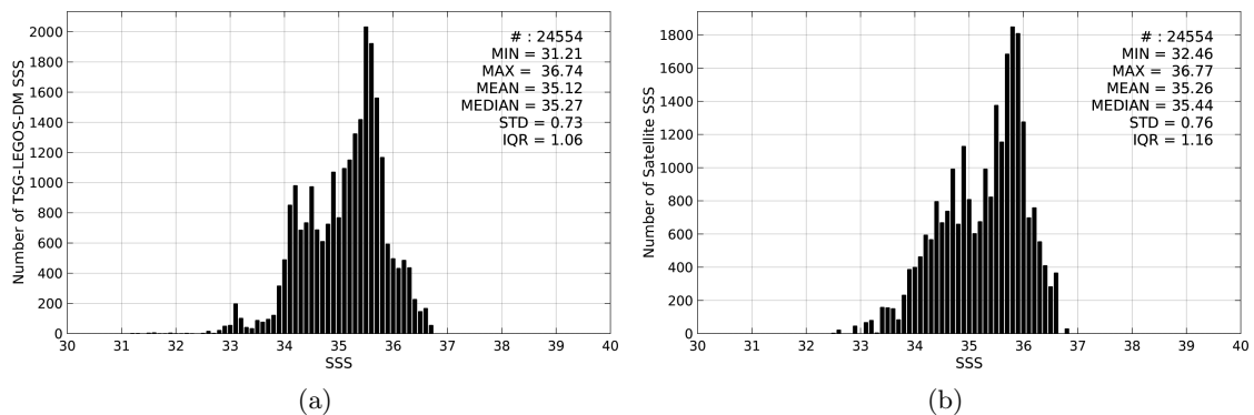
Figure 2: Histograms of SSS from TSG-LEGOS-DM (a) and Aquarius-L3-JPL-V4-MONTHLY (b) considering all match-up pairs per bins of 0.1 over the Indian Ocean Pi-MEP region and for the full satellite product period.
