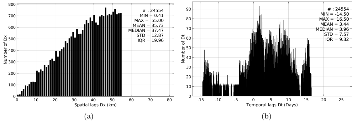
Figure 5: Histograms of the spatial (a) and temporal (b) lags between the time of the TSG-LEGOS-DM measurements and the date of the corresponding Aquarius-L3-JPL-V4-MONTHLY SSS product.
