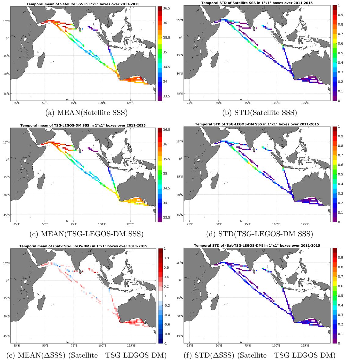
Figure 6: Temporal mean (left) and STD (right) of SSS from Aquarius-L3-JPL-V4-MONTHLY (top), TSG-LEGOS-DM (middle), and of \Delta SSS (Satellite - TSG-LEGOS-DM). Only match-up pairs are used to generate these maps.
