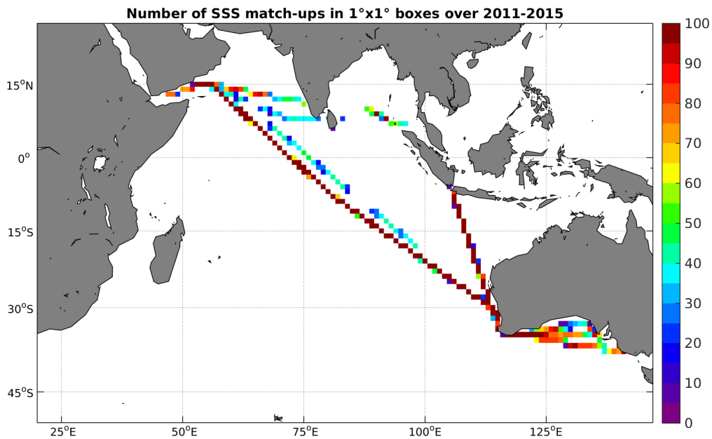
Figure 4: Number of SSS match-ups between TSG-LEGOS-DM SSS and the Aquarius-L3-JPL-V4-MONTHLY SSS product for the Indian Ocean Pi-MEP region over 1^\circ \times 1^\circ boxes and for the full satellite product period.
