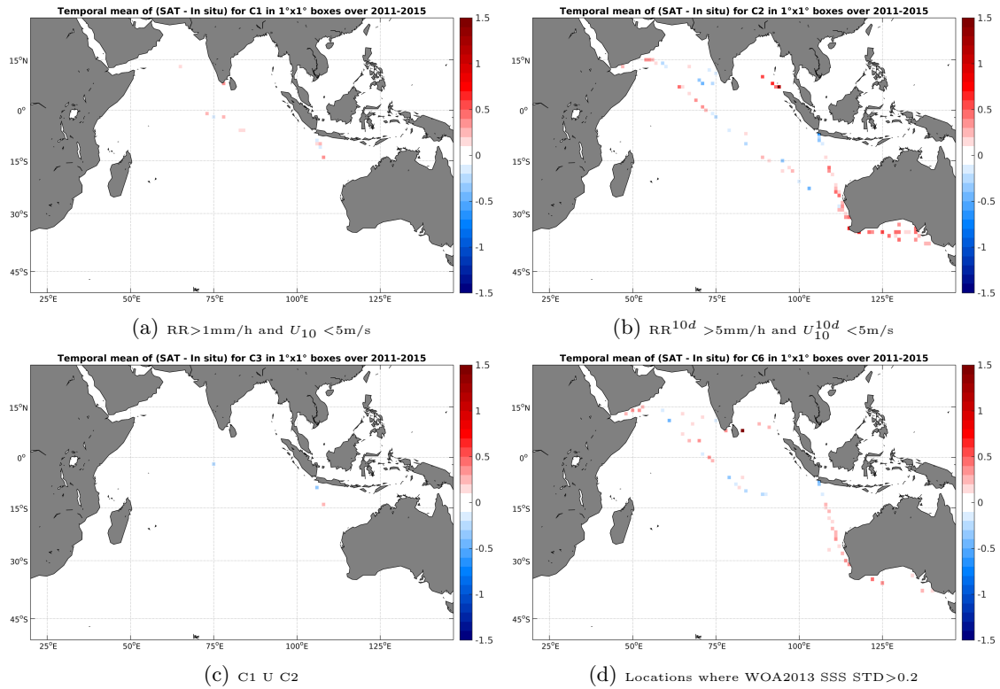
Figure 12: Temporal mean gridded over spatial boxes of size 1^\circ \times 1^\circ of \Delta SSS (Aquarius-L3-JPL-V4-MONTHLY - TSG-LEGOS-DM) for 4 different subdatasets corresponding to:RR > 1mm/h and U_{10} < 5 m/s (a), RR^{10d} > 5 mm/h and U_{10}^{10d} < 5 m/s (b), C1 U C2 (c),Locations where WOA2013 SSS STD > 0.2 (d).
