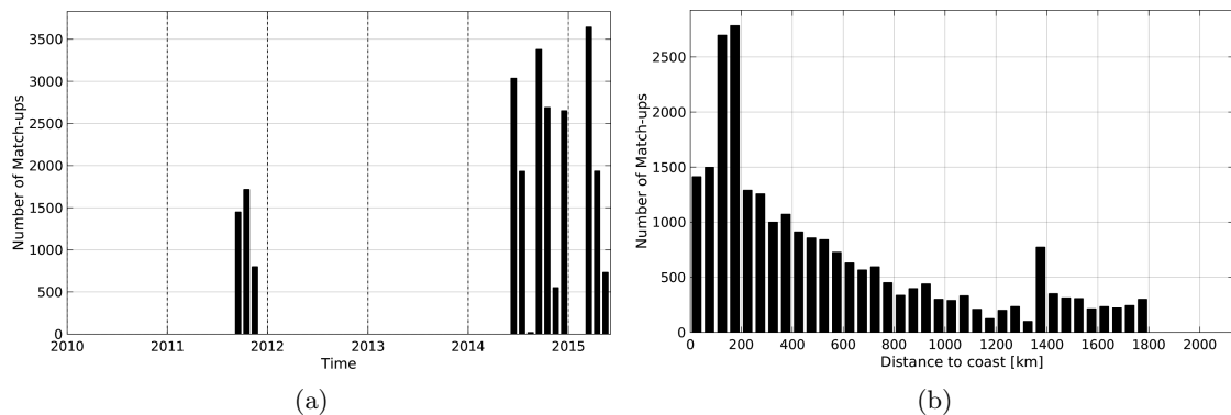
Figure 1: Number of match-ups between TSG-LEGOS-DM and Aquarius-L3-JPL-V4-MONTHLY SSS as a function of time (a) and as function of the distance to coast (b) over the Indian Ocean Pi-MEP region and for the full satellite product period.
