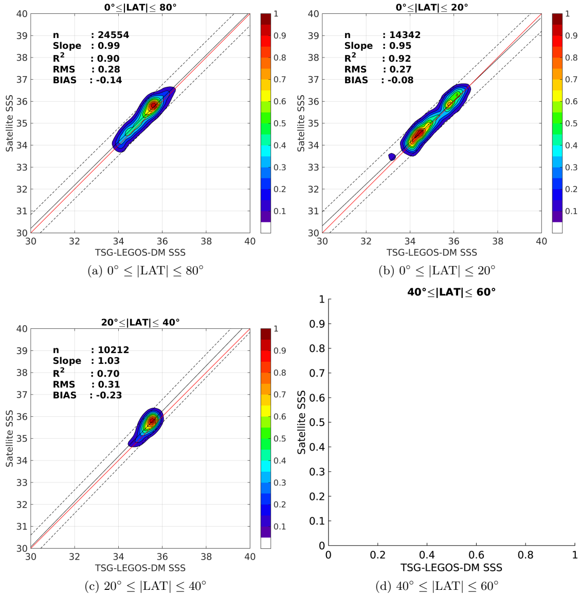
Figure 9: Contour maps of the concentration of Aquarius-L3-JPL-V4-MONTHLY SSS (y-axis) versus TSG-LEGOS-DM SSS (x-axis) at match-up pairs for different latitude bands. For each plot, the red line shows x=y . The black thin and dashed lines indicate a linear fit through the data cloud and the \pm 95\% confidence levels, respectively. The number match-up pairs n , the slope and R^2 coefficient of the linear fit, the root mean square (RMS) and the mean bias between satellite and in situ data are indicated for each latitude band in each plots.
