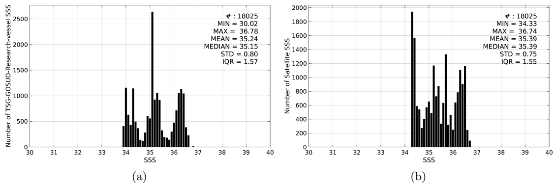
Figure 2: Histograms of SSS from TSG-GOSUD-Research-vessel (a) and Aquarius-L3-JPL-V4-MONTHLY (b) considering all match-up pairs per bins of 0.1 over the Indian Ocean Pi-MEP region and for the full satellite product period.
