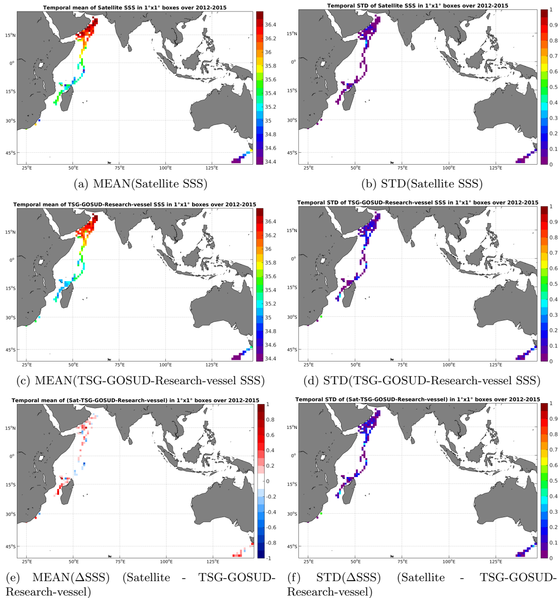
Figure 6: Temporal mean (left) and STD (right) of SSS from Aquarius-L3-JPL-V4-MONTHLY (top), TSG-GOSUD-Research-vessel (middle), and of \Delta SSS (Satellite - TSG-GOSUD-Research-vessel). Only match-up pairs are used to generate these maps.
