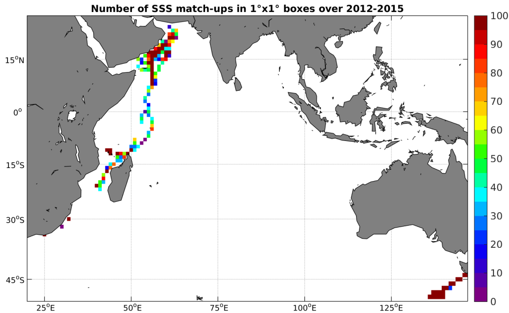
Figure 4: Number of SSS match-ups between TSG-GOSUD-Research-vessel SSS and the Aquarius-L3-JPL-V4-MONTHLY SSS product for the Indian Ocean Pi-MEP region over 1^\circ \times 1^\circ boxes and for the full satellite product period.
