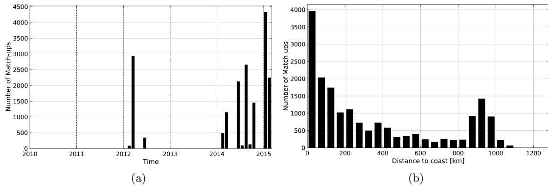
Figure 1: Number of match-ups between TSG-GOSUD-Research-vessel and Aquarius-L3-JPL-V4-MONTHLY SSS as a function of time (a) and as function of the distance to coast (b) over the Indian Ocean Pi-MEP region and for the full satellite product period.
