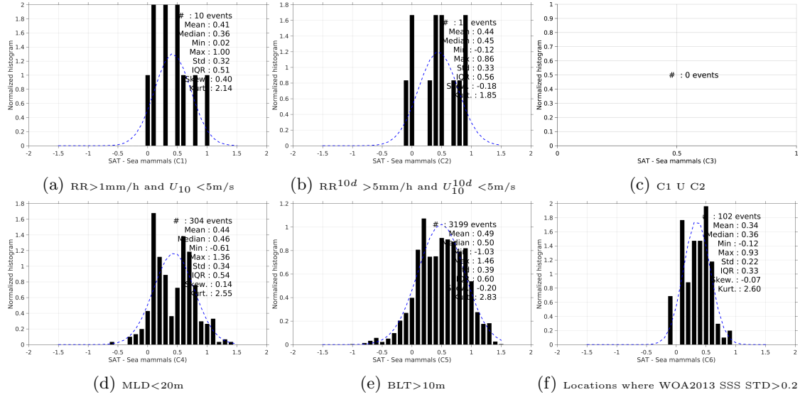
Figure 13: Normalized histogram of \Delta SSS (Aquarius-L3-JPL-V4-MONTHLY - Sea mammals) for 6 different subdatasets corresponding to: RR > 1mm/h and U_{10} < 5 m/s (a), RR 10d > 5mm/h and U_{10}^{10d} < 5 m/s (b), C1 U C2 (c), MLD < 20m (d), BLT > 10m (e), Locations where WOA2013 SSS STD > 0.2 (f).
