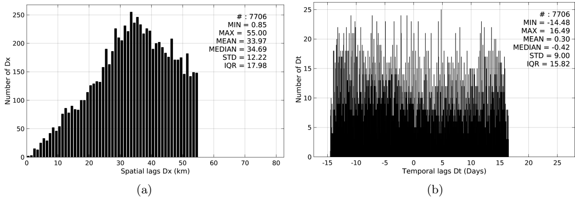
Figure 5: Histograms of the spatial (a) and temporal (b) lags between the time of the Sea mammals measurements and the date of the corresponding Aquarius-L3-JPL-V4-MONTHLY SSS product.
