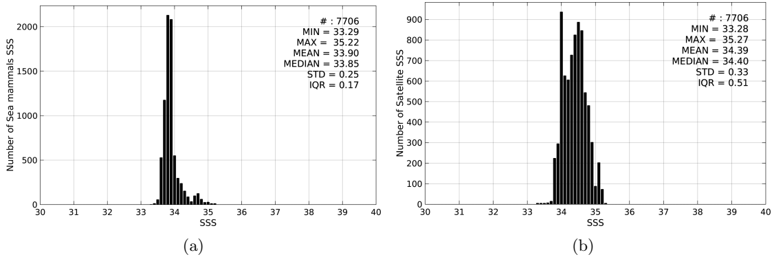
Figure 2: Histograms of SSS from Sea mammals (a) and Aquarius-L3-JPL-V4-MONTHLY (b) considering all match-up pairs per bins of 0.1 over the Indian Ocean Pi-MEP region and for the full satellite product period.
