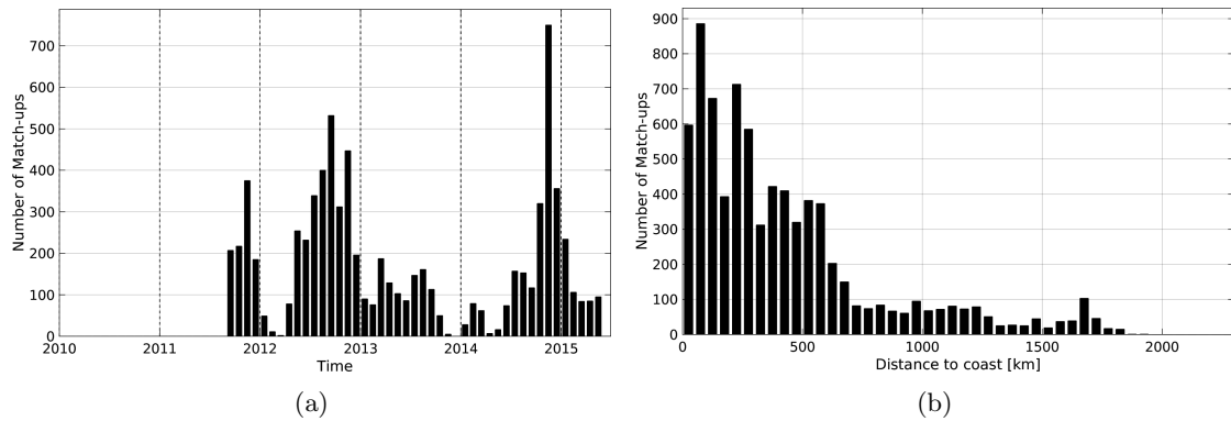
Figure 1: Number of match-ups between Sea mammals and Aquarius-L3-JPL-V4-MONTHLY SSS as a function of time (a) and as function of the distance to coast (b) over the Indian Ocean Pi-MEP region and for the full satellite product period.
