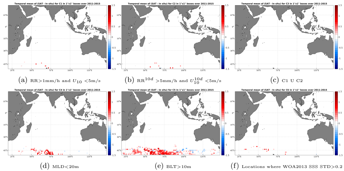
Figure 12: Temporal mean gridded over spatial boxes of size 1^\circ \times 1^\circ of \Delta SSS (Aquarius-L3-JPL-V4-MONTHLY - Sea mammals) for 6 different subdatasets corresponding to:RR>1mm/h and U_{10} < 5\text{m/s} (a), RR^{10d} > 5\text{mm/h} and U_{10}^{10d} < 5\text{m/s} (b), C1 U C2 (c),MLD<20m (d),BLT>10m (e),Locations where WOA2013 SSS STD>0.2 (f).
