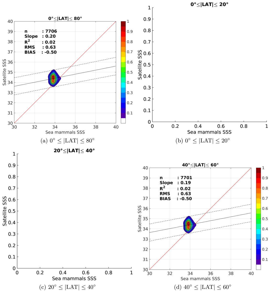
Figure 9: Contour maps of the concentration of Aquarius-L3-JPL-V4-MONTHLY SSS (y-axis) versus Sea mammals SSS (x-axis) at match-up pairs for different latitude bands. For each plot, the red line shows x=y . The black thin and dashed lines indicate a linear fit through the data cloud and the \pm 95\% confidence levels, respectively. The number match-up pairs n , the slope and R^2 coefficient of the linear fit, the root mean square (RMS) and the mean bias between satellite and in situ data are indicated for each latitude band in each plots.
