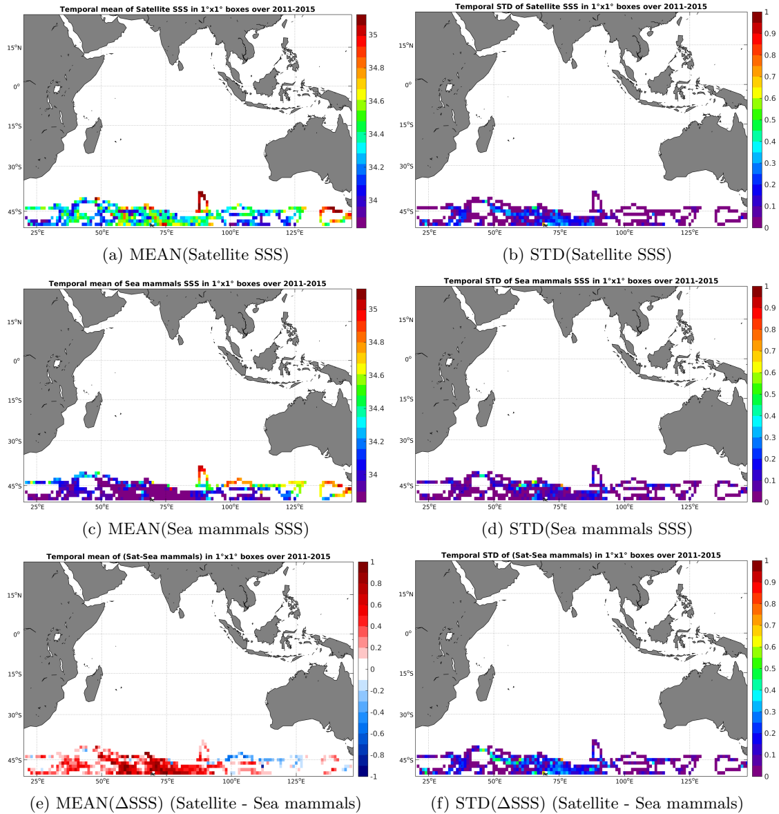
Figure 6: Temporal mean (left) and STD (right) of SSS from Aquarius-L3-JPL-V4-MONTHLY (top), Sea mammals (middle), and of \Delta SSS (Satellite - Sea mammals). Only match-up pairs are used to generate these maps.
