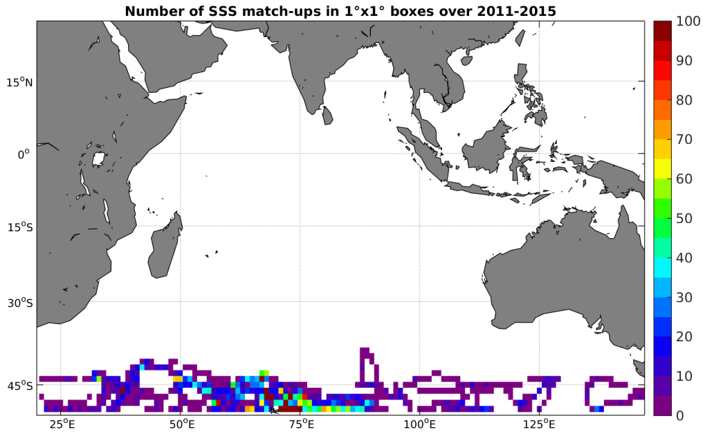
Figure 4: Number of SSS match-ups between Sea mammals SSS and the Aquarius-L3-JPL-V4-MONTHLY SSS product for the Indian Ocean Pi-MEP region over 1°x1° boxes and for the full satellite product period.
