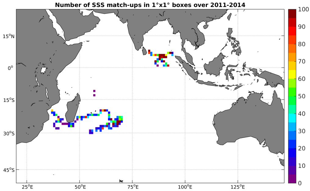
Figure 3: Number of SSS match-ups between Surface drifters SSS and the Aquarius-L3-JPL-V4-MONTHLY SSS product for the Indian Ocean Pi-MEP region over 1°x1° boxes and for the full satellite product period.
