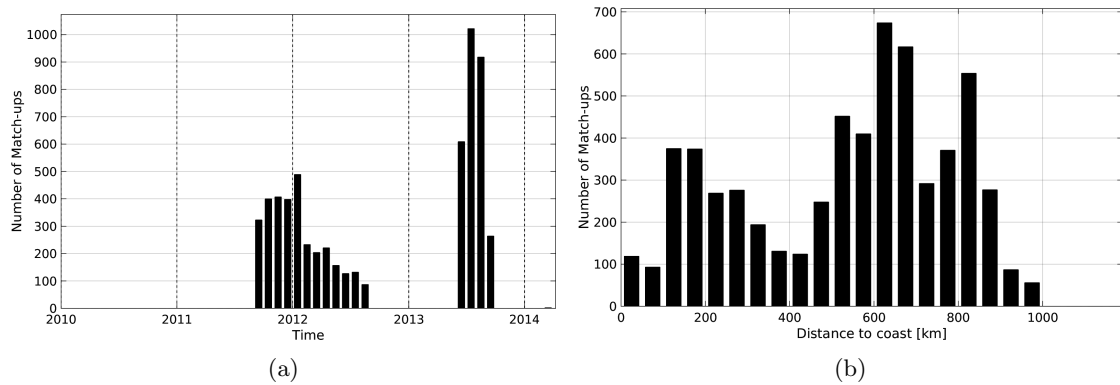
Figure 1: Number of match-ups between Surface drifters and Aquarius-L3-JPL-V4-MONTHLY SSS as a function of time (a) and as function of the distance to coast (b) over the Indian Ocean Pi-MEP region and for the full satellite product period.
