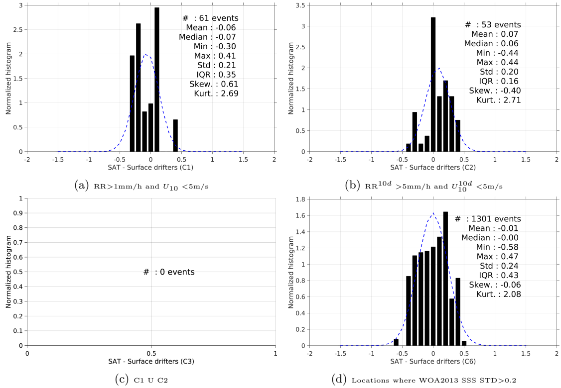
Figure 12: Normalized histogram of \Delta\text{SSS} (Aquarius-L3-JPL-V4-MONTHLY - Surface drifters) for 6 different subdatasets corresponding to: RR > 1\text{mm/h} and U_{10} < 5\text{m/s} (a), RR^{10d} > 5\text{mm/h} and U_{10}^{10d} < 5\text{m/s} (b), C1 U C2 (c), Locations where WOA2013 SSS STD > 0.2 (d).
