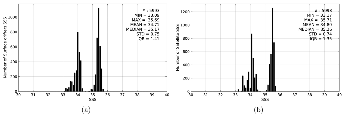
Figure 2: Histograms of SSS from Surface drifters (a) and Aquarius-L3-JPL-V4-MONTHLY (b) considering all match-up pairs per bins of 0.1 over the Indian Ocean Pi-MEP region and for the full satellite product period.
