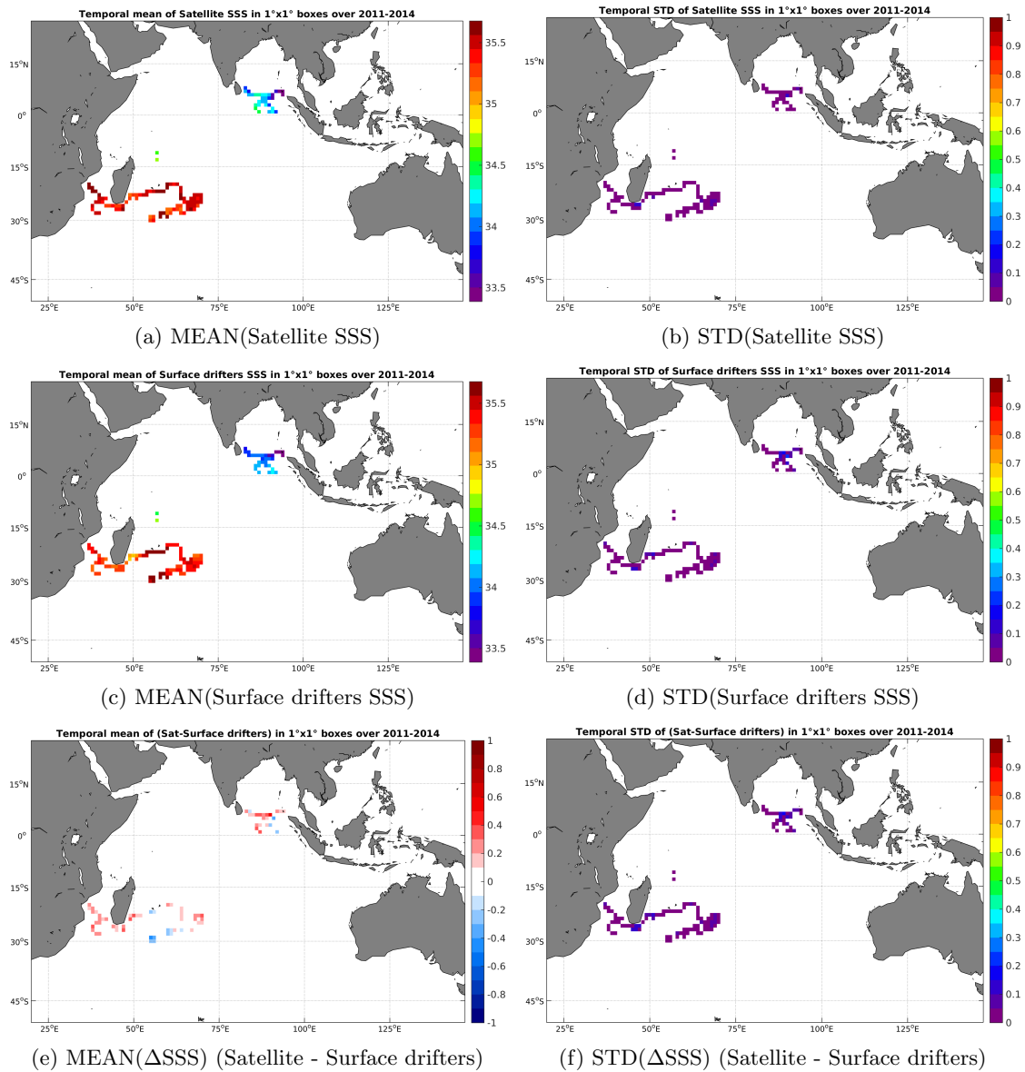
Figure 5: Temporal mean (left) and STD (right) of SSS from Aquarius-L3-JPL-V4-MONTHLY (top), Surface drifters (middle), and of \Delta SSS (Satellite - Surface drifters). Only match-up pairs are used to generate these maps.
