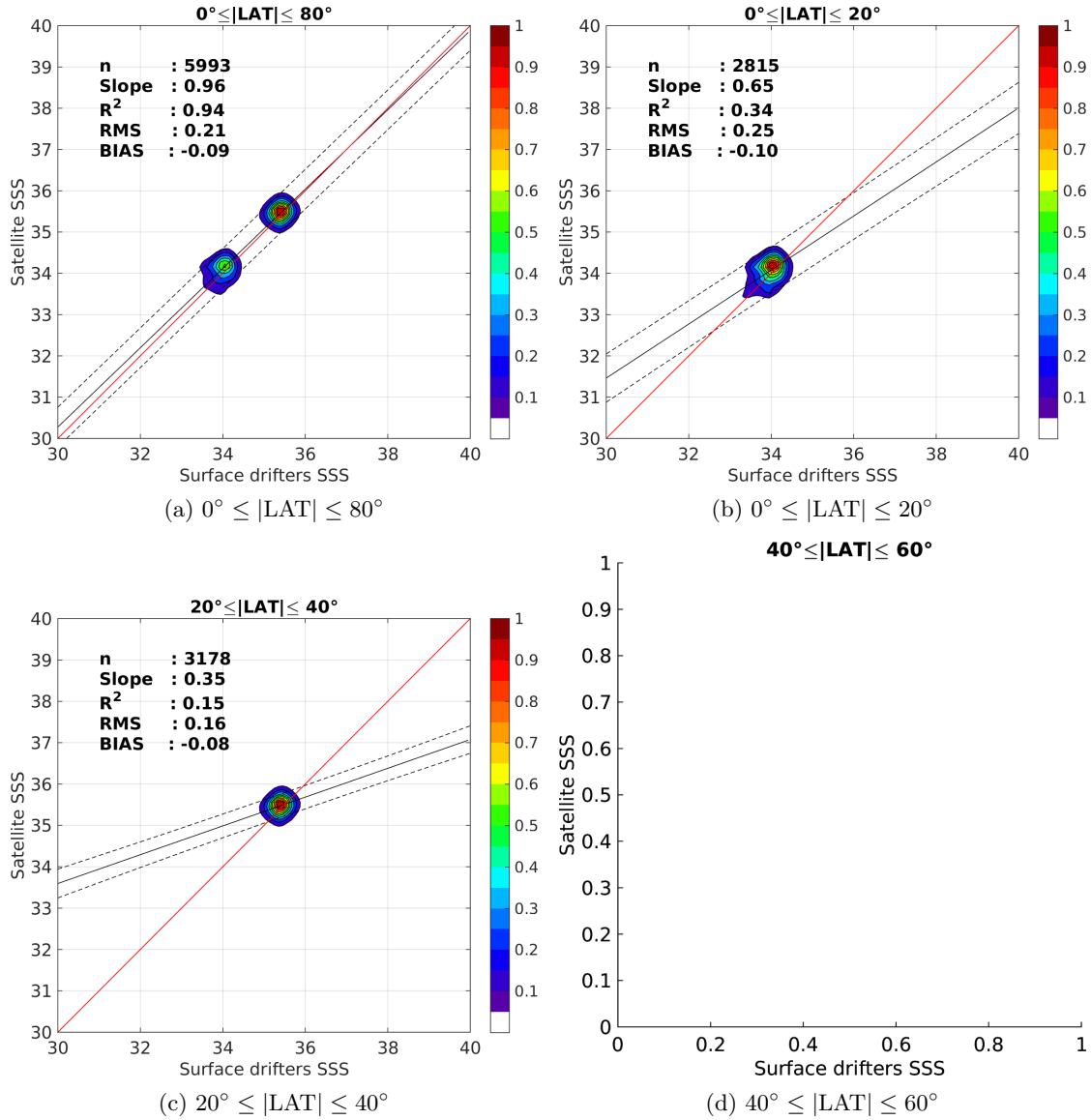
Figure 8: Contour maps of the concentration of Aquarius-L3-JPL-V4-MONTHLY SSS (y-axis) versus Surface drifters SSS (x-axis) at match-up pairs for different latitude bands. For each plot, the red line shows x=y . The black thin and dashed lines indicate a linear fit through the data cloud and the \pm 95\% confidence levels, respectively. The number match-up pairs n , the slope and R^2 coefficient of the linear fit, the root mean square (RMS) and the mean bias between satellite and in situ data are indicated for each latitude band in each plots.
