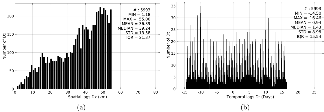
Figure 4: Histograms of the spatial (a) and temporal (b) lags between the time of the Surface drifters measurements and the date of the corresponding Aquarius-L3-JPL-V4-MONTHLY SSS product.
