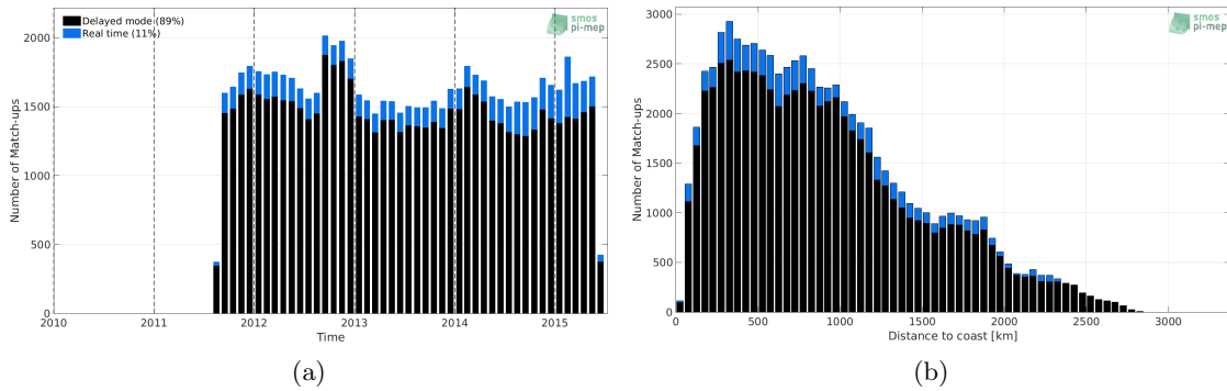
Figure 1: Number of match-ups between Argo and Aquarius SSS L2-AVERAGED OR v5 (NASA-GSFC) SSS as a function of time (a) and as function of the distance to coast (b) over the Indian Ocean Pi-MEP region and for the full satellite product period.
