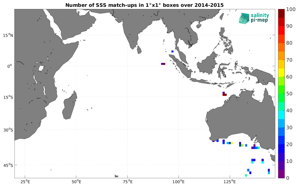
Figure 5: Number of SSS match-ups between TSG (SAMOS) SSS and the Aquarius SSS L2 OR v5 (NASA-GSFC) SSS product for the Indian Ocean Pi-MEP region over 1^\circ \times 1^\circ boxes and for the full satellite product period.
