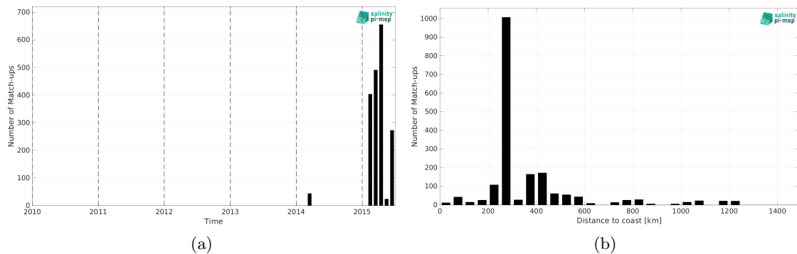
Figure 2: Number of match-ups between TSG (SAMOS) and Aquarius SSS L2 OR v5 (NASA-GSFC) SSS as a function of time (a) and as function of the distance to coast (b) over the Indian Ocean Pi-MEP region and for the full satellite product period.
