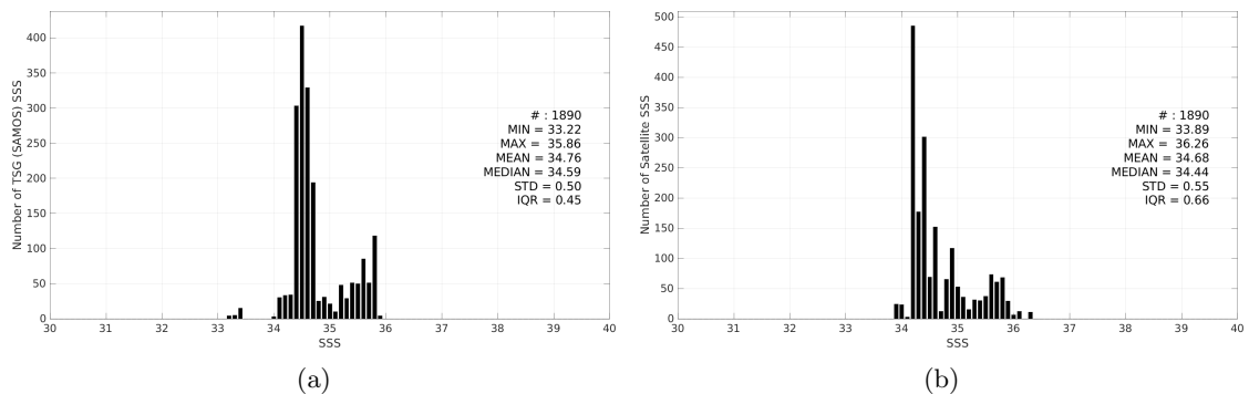
Figure 3: Histograms of SSS from TSG (SAMOS) (a) and Aquarius SSS L2 OR v5 (NASA-GSFC) (b) considering all match-up pairs per bins of 0.1 over the Indian Ocean Pi-MEP region and for the full satellite product period.
