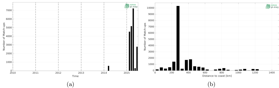
Figure 1: Number of match-ups between TSG (SAMOS) and Aquarius SSS L2 OR v5 (NASA-GSFC) SSS as a function of time (a) and as function of the distance to coast (b) over the Indian Ocean Pi-MEP region and for the full satellite product period.
