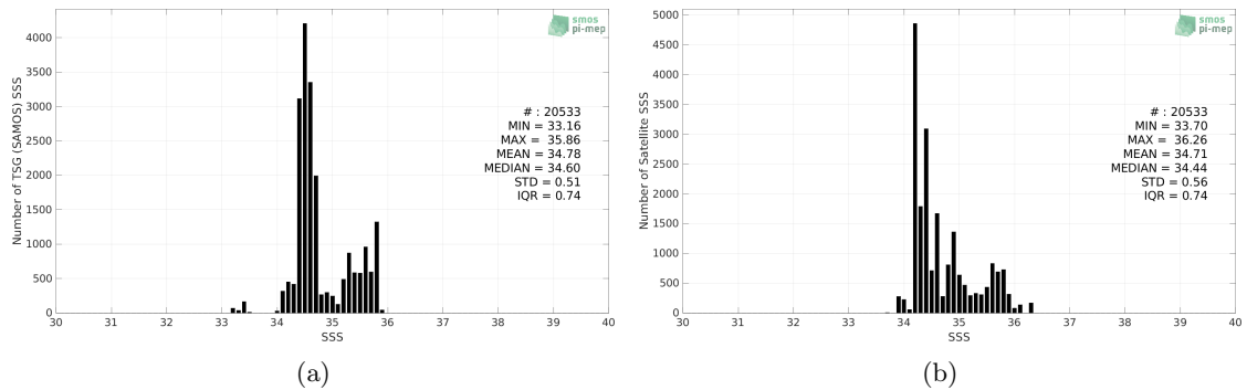
Figure 2: Histograms of SSS from TSG (SAMOS) (a) and Aquarius SSS L2 OR v5 (NASA-GSFC) (b) considering all match-up pairs per bins of 0.1 over the Indian Ocean Pi-MEP region and for the full satellite product period.
