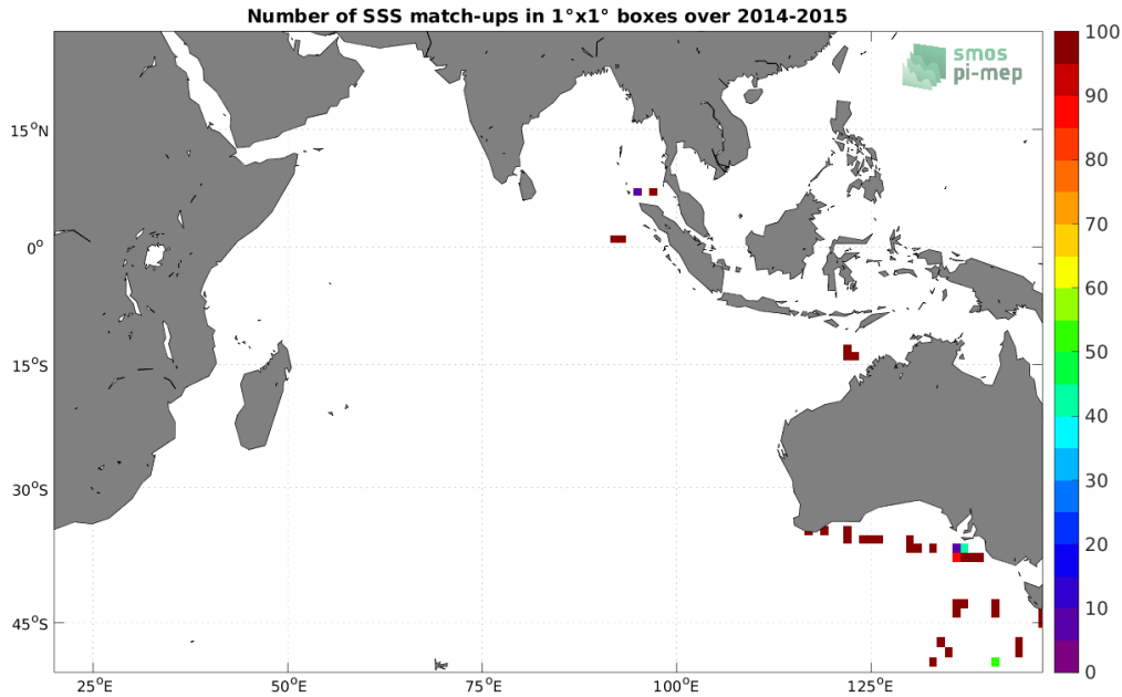
Figure 4: Number of SSS match-ups between TSG (SAMOS) SSS and the Aquarius SSS L2 OR v5 (NASA-GSFC) SSS product for the Indian Ocean Pi-MEP region over 1^\circ \times 1^\circ boxes and for the full satellite product period.
