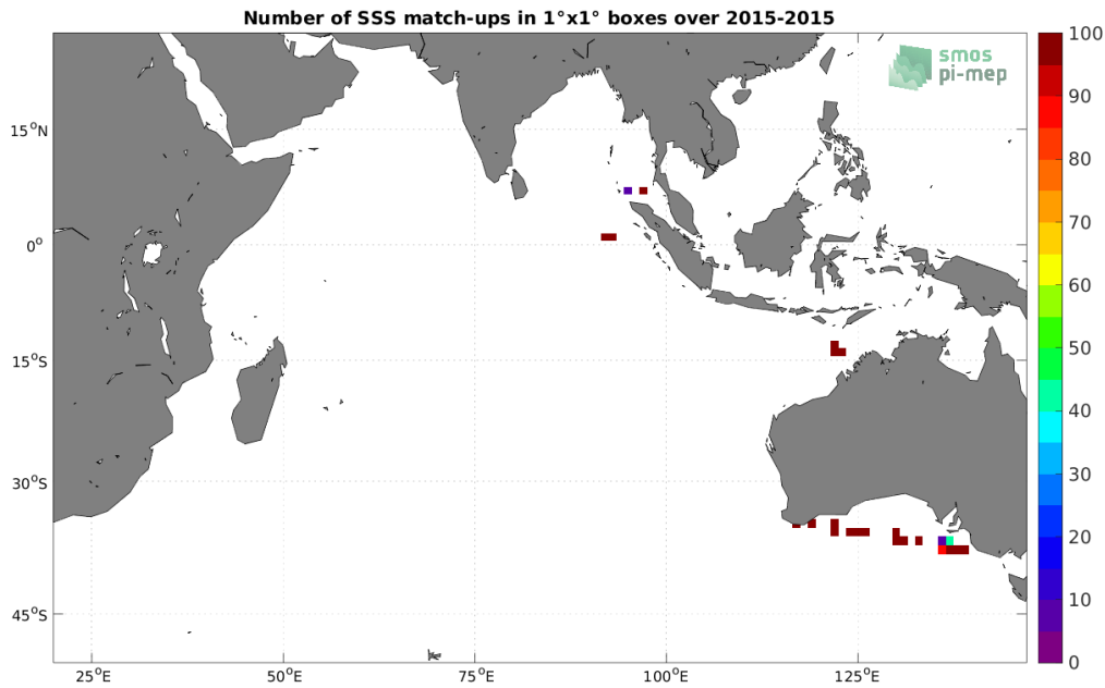
Figure 4: Number of SSS match-ups between TSG (SAMOS) SSS and the Aquarius SSS L2 OR v5 (NASA-GSFC) SSS product for the Indian Ocean Pi-MEP region over 1^\circ \times 1^\circ boxes and for the full satellite product period.
