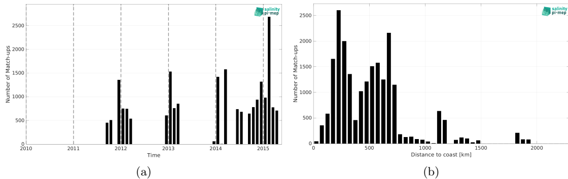
Figure 2: Number of match-ups between TSG (LEGOS-DM) and Aquarius SSS L2 OR v5 (NASA-GSFC) SSS as a function of time (a) and as function of the distance to coast (b) over the Indian Ocean Pi-MEP region and for the full satellite product period.
