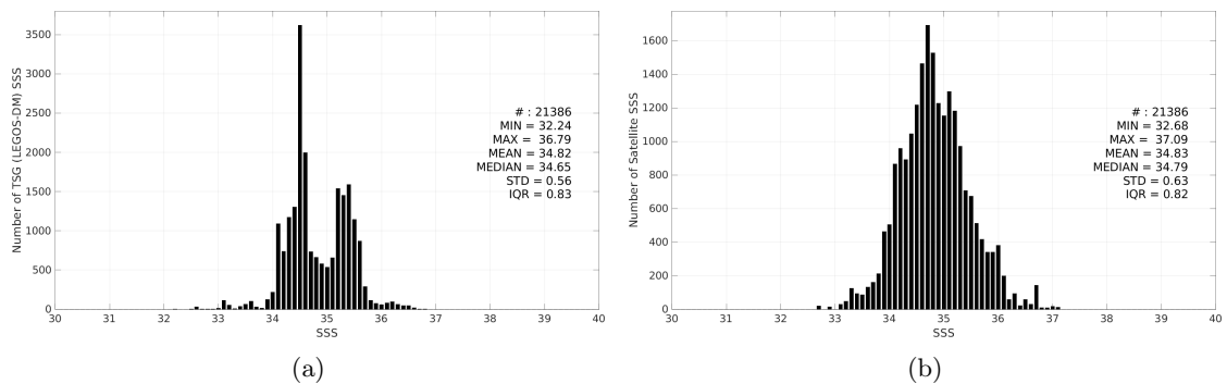
Figure 3: Histograms of SSS from TSG (LEGOS-DM) (a) and Aquarius SSS L2 OR v5 (NASA-GSFC) (b) considering all match-up pairs per bins of 0.1 over the Indian Ocean Pi-MEP region and for the full satellite product period.
