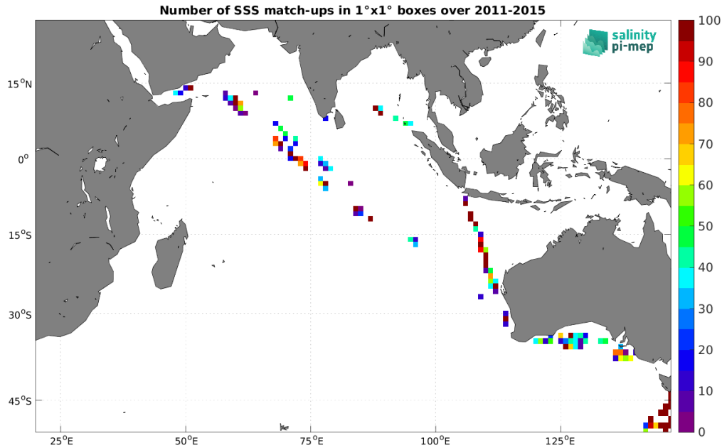
Figure 5: Number of SSS match-ups between TSG (LEGOS-DM) SSS and the Aquarius SSS L2 OR v5 (NASA-GSFC) SSS product for the Indian Ocean Pi-MEP region over 1^\circ \times 1^\circ boxes and for the full satellite product period.
