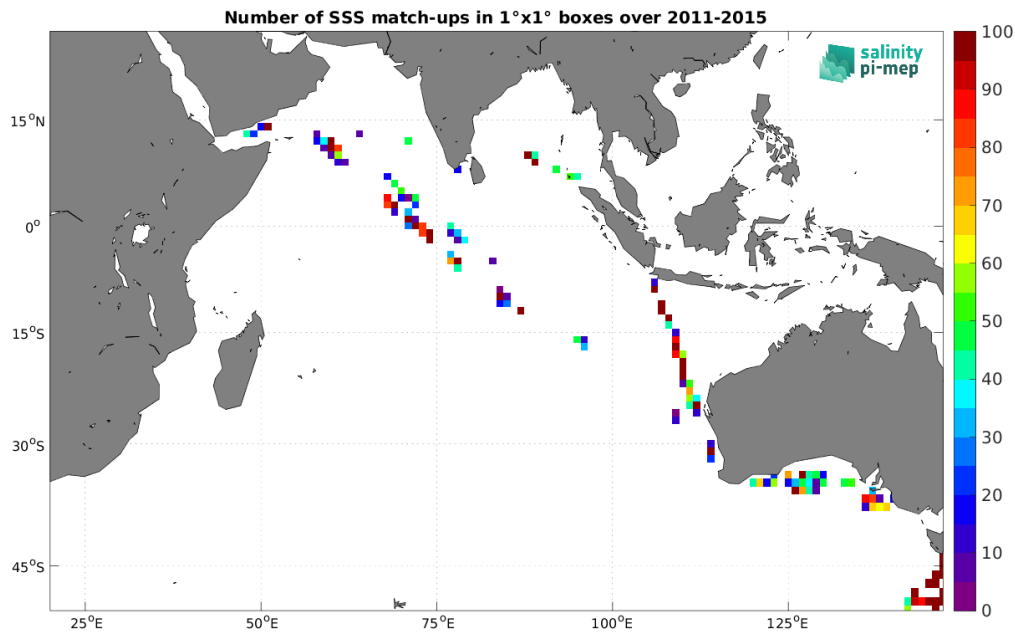
Figure 4: Number of SSS match-ups between TSG (LEGOS-DM) SSS and the Aquarius SSS L2 OR v5 (NASA-GSFC) SSS product for the Indian Ocean Pi-MEP region over 1^\circ \times 1^\circ boxes and for the full satellite product period.
