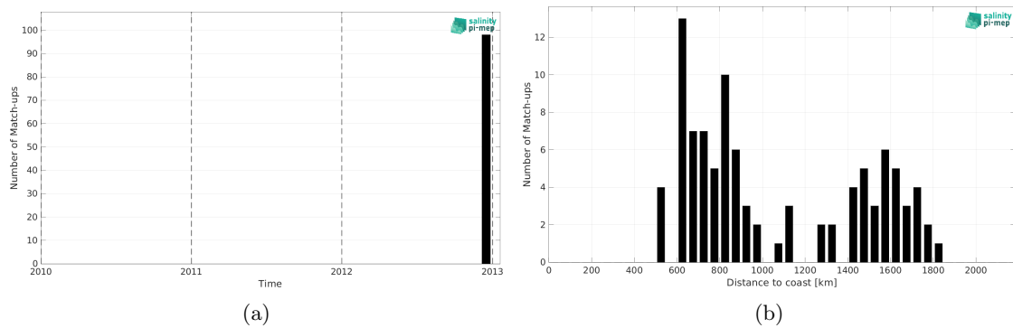
Figure 2: Number of match-ups between TSG (GOSUD-Sailing-ship) and Aquarius SSS L2 OR v5 (NASA-GSFC) SSS as a function of time (a) and as function of the distance to coast (b) over the Indian Ocean Pi-MEP region and for the full satellite product period.
