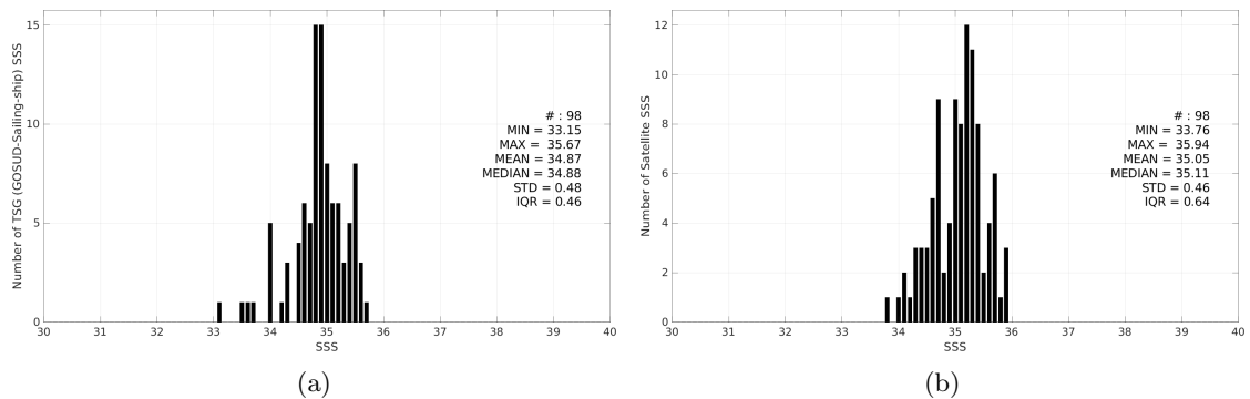
Figure 3: Histograms of SSS from TSG (GOSUD-Sailing-ship) (a) and Aquarius SSS L2 OR v5 (NASA-GSFC) (b) considering all match-up pairs per bins of 0.1 over the Indian Ocean Pi-MEP region and for the full satellite product period.
