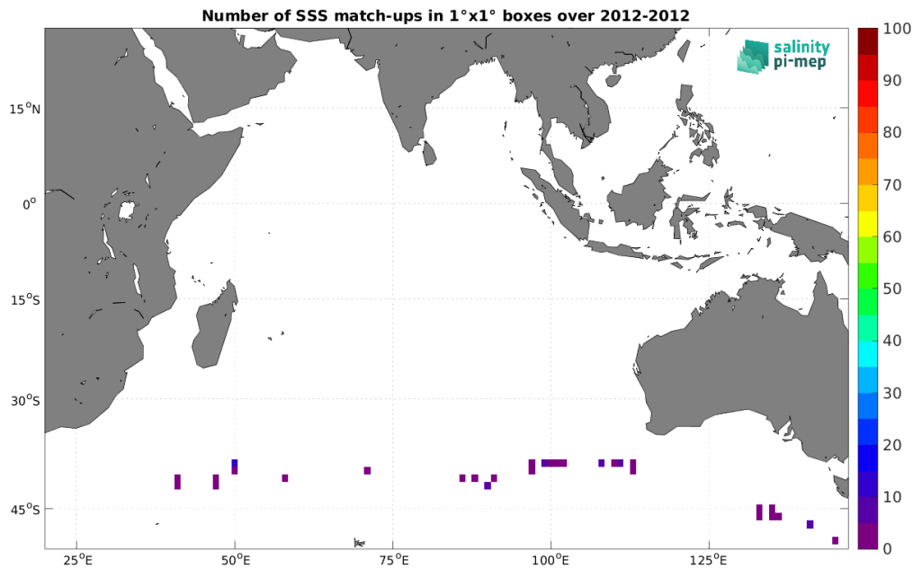
Figure 4: Number of SSS match-ups between TSG (GOSUD-Sailing-ship) SSS and the Aquarius SSS L2 OR v5 (NASA-GSFC) SSS product for the Indian Ocean Pi-MEP region over 1^\circ \times 1^\circ boxes and for the full satellite product period.
