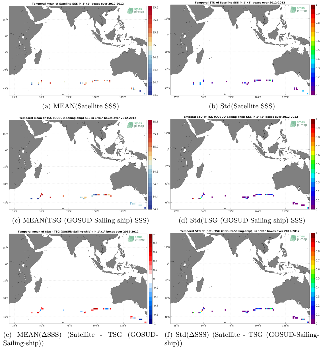
Figure 6: Temporal mean (left) and Std (right) of SSS from Aquarius SSS L2 OR v5 (NASA-GSFC) (top), TSG (GOSUD-Sailing-ship) (middle), and of \Delta SSS (Satellite - TSG (GOSUD-Sailing-ship)). Only match-up pairs are used to generate these maps.
