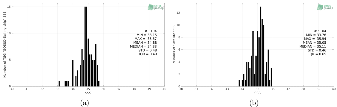
Figure 2: Histograms of SSS from TSG (GOSUD-Sailing-ship) (a) and Aquarius SSS L2 OR v5 (NASA-GSFC) (b) considering all match-up pairs per bins of 0.1 over the Indian Ocean Pi-MEP region and for the full satellite product period.
