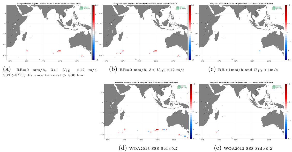
Figure 12: Temporal mean gridded over spatial boxes of size 1^\circ \times 1^\circ of \Delta SSS (Aquarius SSS L2 OR v5 (NASA-GSFC) - TSG (GOSUD-Sailing-ship)) for 5 different subdatasets corresponding to:RR=0 mm/h, 3 < U_{10} < 12 m/s, SST >5^\circ C, distance to coast > 800 km (a), RR=0 mm/h, 3 < U_{10} < 12 m/s (b), RR >1 mm/h and U_{10} < 4 m/s (c), WOA2013 SSS Std <0.2 (d), WOA2013 SSS Std >0.2 (e).
