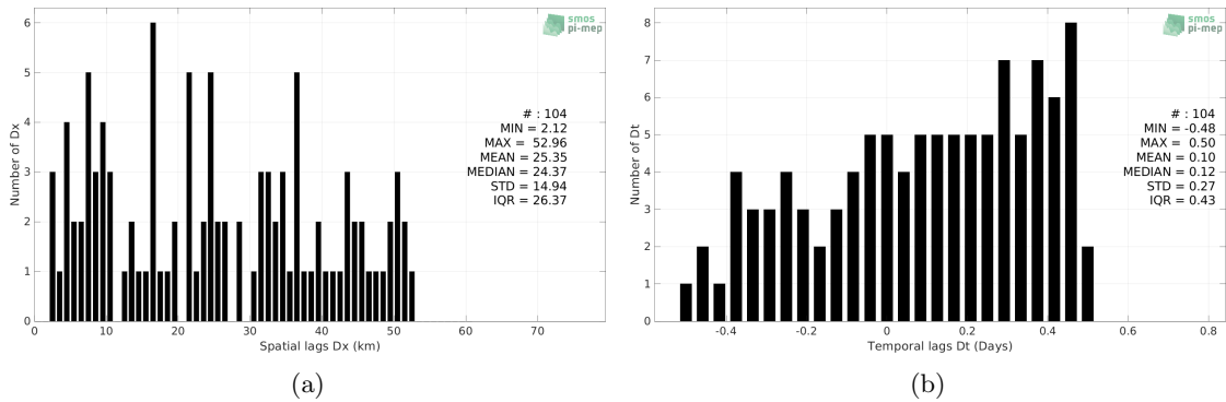
Figure 5: Histograms of the spatial (a) and temporal (b) lags between the location/time of the TSG (GOSUD-Sailing-ship) measurement and the date of the corresponding Aquarius SSS L2 OR v5 (NASA-GSFC) SSS pixel.
