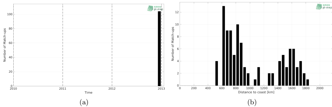
Figure 1: Number of match-ups between TSG (GOSUD-Sailing-ship) and Aquarius SSS L2 OR v5 (NASA-GSFC) SSS as a function of time (a) and as function of the distance to coast (b) over the Indian Ocean Pi-MEP region and for the full satellite product period.
