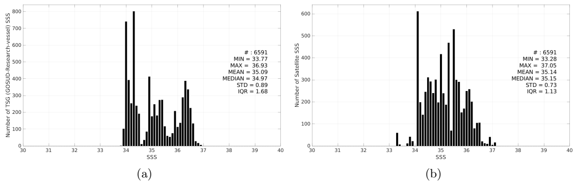
Figure 3: Histograms of SSS from TSG (GOSUD-Research-vessel) (a) and Aquarius SSS L2 OR v5 (NASA-GSFC) (b) considering all match-up pairs per bins of 0.1 over the Indian Ocean Pi-MEP region and for the full satellite product period.
