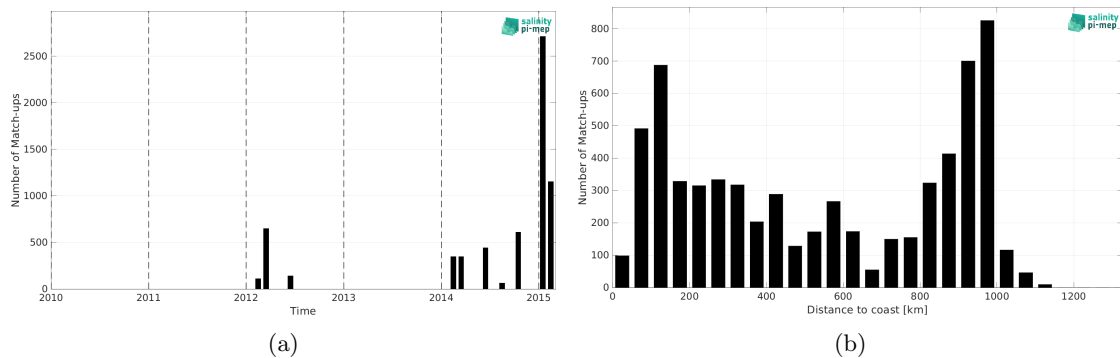
Figure 2: Number of match-ups between TSG (GOSUD-Research-vessel) and Aquarius SSS L2 OR v5 (NASA-GSFC) SSS as a function of time (a) and as function of the distance to coast (b) over the Indian Ocean Pi-MEP region and for the full satellite product period.
