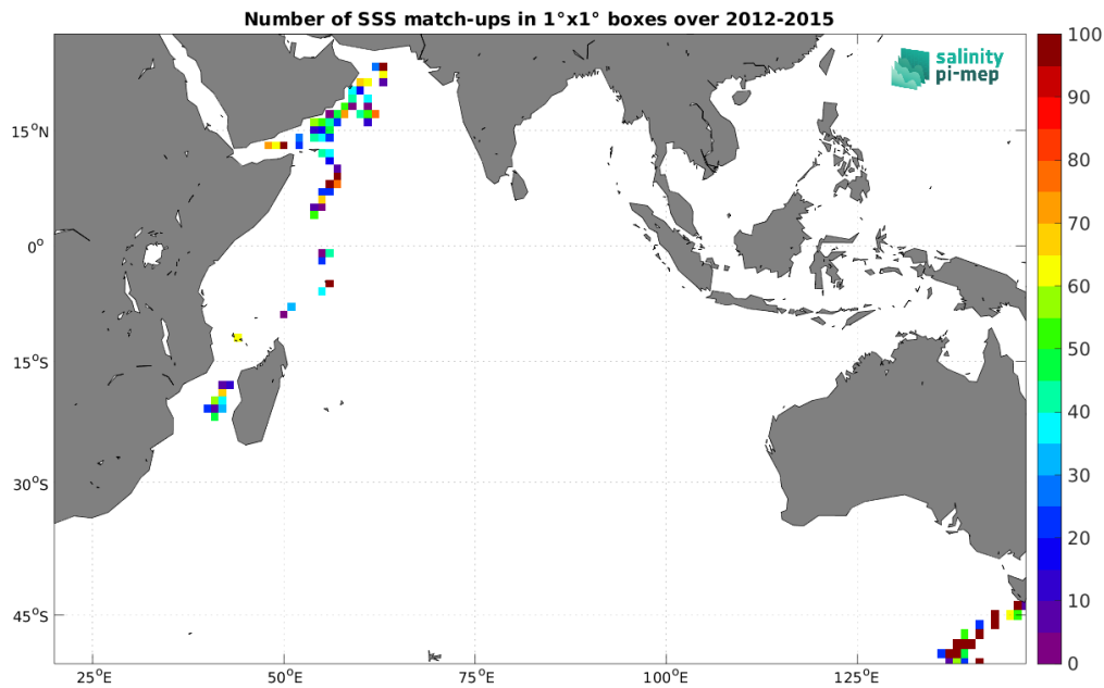
Figure 5: Number of SSS match-ups between TSG (GOSUD-Research-vessel) SSS and the Aquarius SSS L2 OR v5 (NASA-GSFC) SSS product for the Indian Ocean Pi-MEP region over 1^\circ \times 1^\circ boxes and for the full satellite product period.
