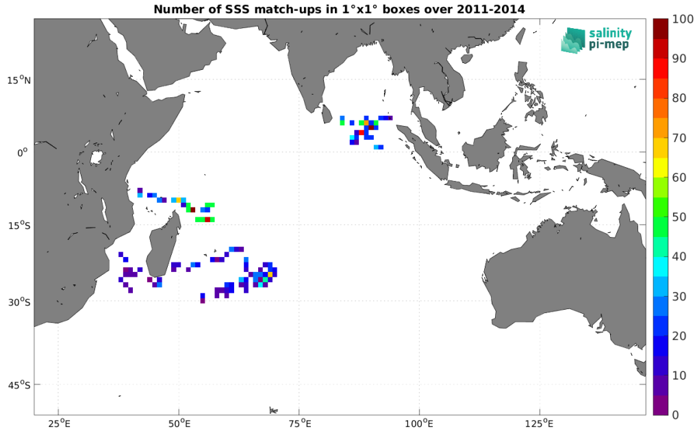
Figure 4: Number of SSS match-ups between Surface drifters SSS and the Aquarius SSS L2 OR v5 (NASA-GSFC) SSS product for the Indian Ocean Pi-MEP region over 1^\circ \times 1^\circ boxes and for the full satellite product period.
