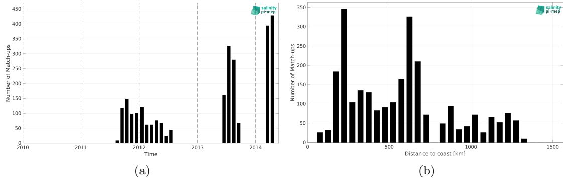
Figure 2: Number of match-ups between Surface drifters and Aquarius SSS L2 OR v5 (NASA-GSFC) SSS as a function of time (a) and as function of the distance to coast (b) over the Indian Ocean Pi-MEP region and for the full satellite product period.
