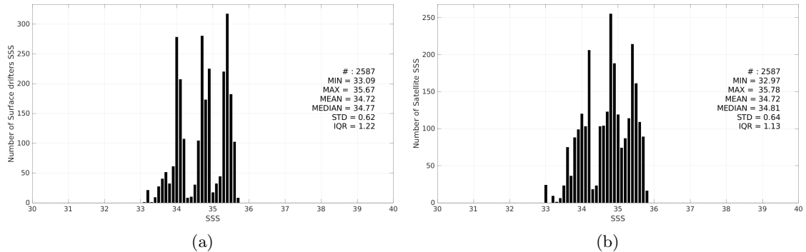
Figure 3: Histograms of SSS from Surface drifters (a) and Aquarius SSS L2 OR v5 (NASA-GSFC) (b) considering all match-up pairs per bins of 0.1 over the Indian Ocean Pi-MEP region and for the full satellite product period.
