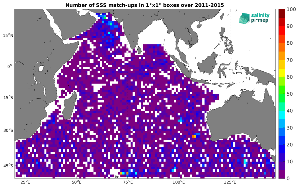
Figure 4: Number of SSS match-ups between Argo SSS and the Aquarius SSS L2 OR v5 (NASA-GSFC) SSS product for the Indian Ocean Pi-MEP region over 1^\circ \times 1^\circ boxes and for the full satellite product period.
