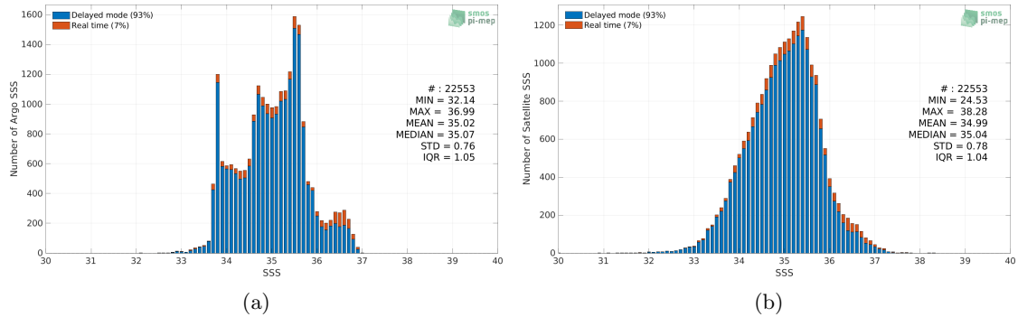
Figure 2: Histograms of SSS from Argo (a) and Aquarius SSS L2 OR v5 (NASA-GSFC) (b) considering all match-up pairs per bins of 0.1 over the Indian Ocean Pi-MEP region and for the full satellite product period.
