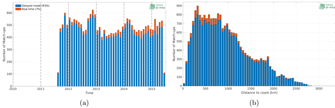
Figure 1: Number of match-ups between Argo and Aquarius SSS L2 OR v5 (NASA-GSFC) SSS as a function of time (a) and as function of the distance to coast (b) over the Indian Ocean Pi-MEP region and for the full satellite product period.
