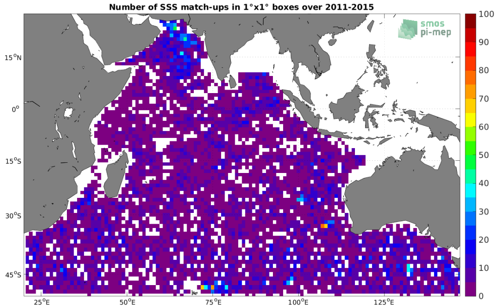
Figure 4: Number of SSS match-ups between Argo SSS and the Aquarius SSS L2 OR v5 (NASA-GSFC) SSS product for the Indian Ocean Pi-MEP region over 1^\circ \times 1^\circ boxes and for the full satellite product period.
