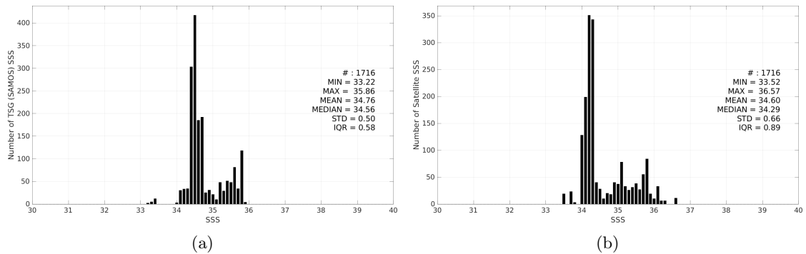
Figure 3: Histograms of SSS from TSG (SAMOS) (a) and Aquarius SSS L2 CAP v5 (JPL) (b) considering all match-up pairs per bins of 0.1 over the Indian Ocean Pi-MEP region and for the full satellite product period.
