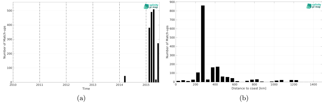
Figure 2: Number of match-ups between TSG (SAMOS) and Aquarius SSS L2 CAP v5 (JPL) SSS as a function of time (a) and as function of the distance to coast (b) over the Indian Ocean Pi-MEP region and for the full satellite product period.
