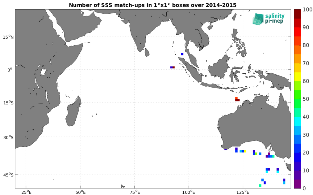
Figure 5: Number of SSS match-ups between TSG (SAMOS) SSS and the Aquarius SSS L2 CAP v5 (JPL) SSS product for the Indian Ocean Pi-MEP region over 1^\circ \times 1^\circ boxes and for the full satellite product period.
