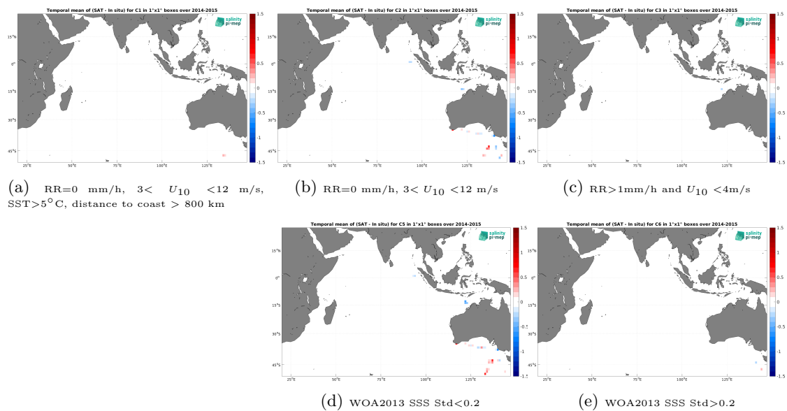
Figure 14: Temporal mean gridded over spatial boxes of size 1^\circ \times 1^\circ of \Delta SSS (Aquarius SSS L2 CAP v5 (JPL) - TSG (SAMOS)) for 5 different subdatasets corresponding to:RR=0 mm/h, 3 < U_{10} < 12 m/s, SST >5^\circ C, distance to coast > 800 km (a), RR=0 mm/h, 3 < U_{10} < 12 m/s (b), RR >1 mm/h and U_{10} < 4 m/s (c), WOA2013 SSS Std <0.2 (d), WOA2013 SSS Std >0.2 (e).
