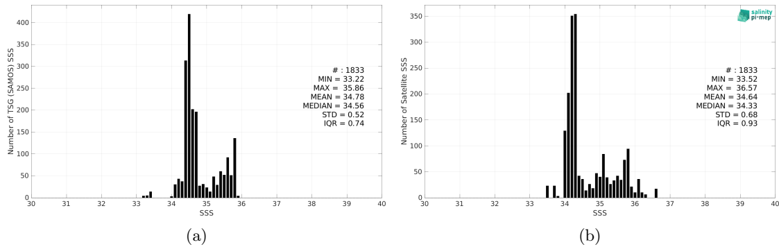
Figure 2: Histograms of SSS from TSG (SAMOS) (a) and Aquarius SSS L2 CAP v5 (JPL) (b) considering all match-up pairs per bins of 0.1 over the Indian Ocean Pi-MEP region and for the full satellite product period.
