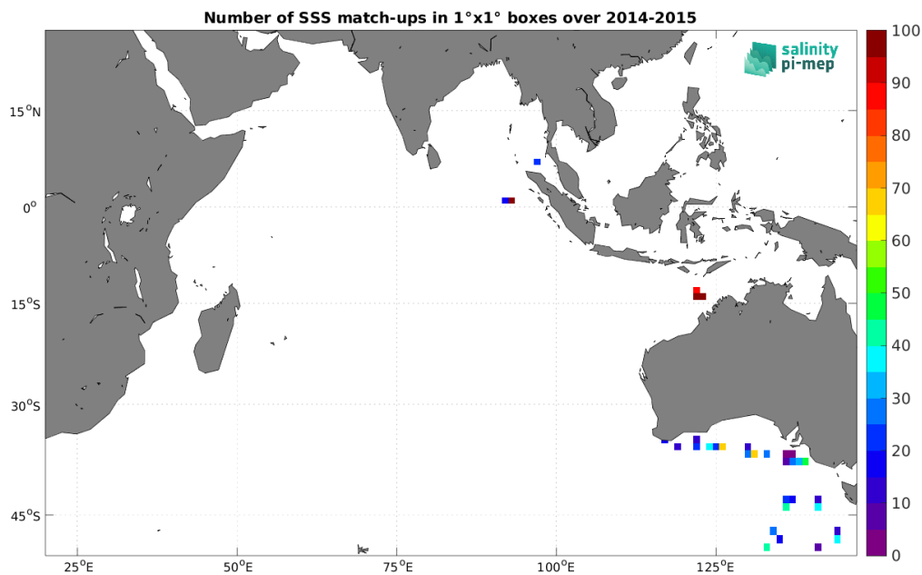
Figure 4: Number of SSS match-ups between TSG (SAMOS) SSS and the Aquarius SSS L2 CAP v5 (JPL) SSS product for the Indian Ocean Pi-MEP region over 1^\circ \times 1^\circ boxes and for the full satellite product period.
