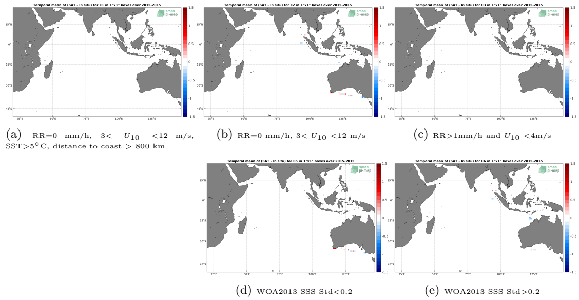
Figure 12: Temporal mean gridded over spatial boxes of size 1^\circ \times 1^\circ of \Delta SSS (Aquarius SSS L2 CAP v5 (JPL) - TSG (SAMOS)) for 5 different subdatasets corresponding to: RR=0 mm/h, 3 < U_{10} < 12 m/s, SST > 5^\circ C , distance to coast > 800 km (a), RR=0 mm/h, 3 < U_{10} < 12 m/s (b), RR > 1 mm/h and U_{10} < 4 m/s (c), WOA2013 SSS Std < 0.2 (d), WOA2013 SSS Std > 0.2 (e).
