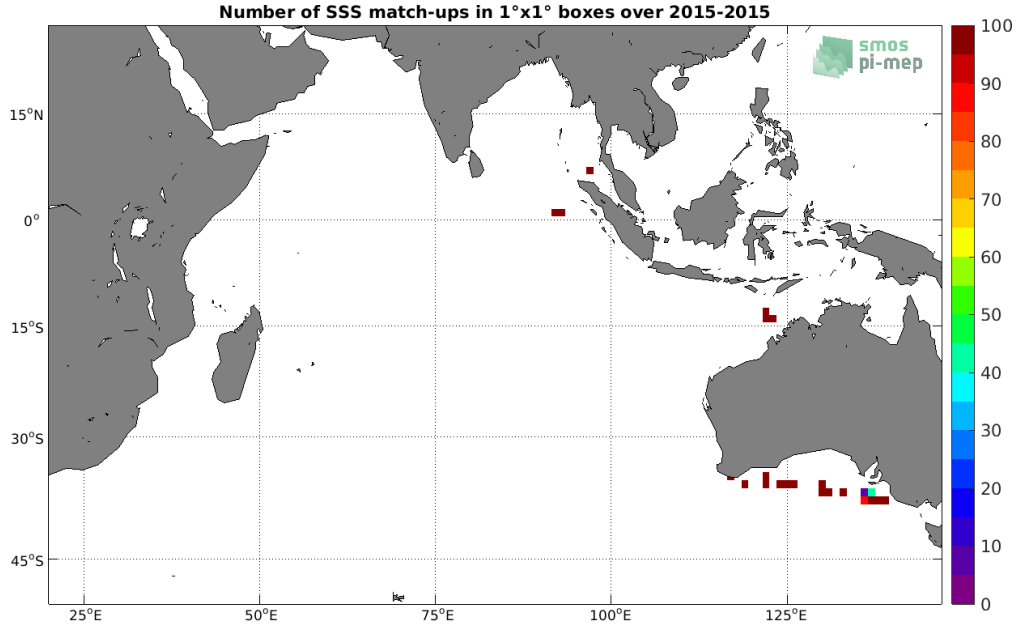
Figure 4: Number of SSS match-ups between TSG (SAMOS) SSS and the Aquarius SSS L2 CAP v5 (JPL) SSS product for the Indian Ocean Pi-MEP region over 1^\circ \times 1^\circ boxes and for the full satellite product period.
