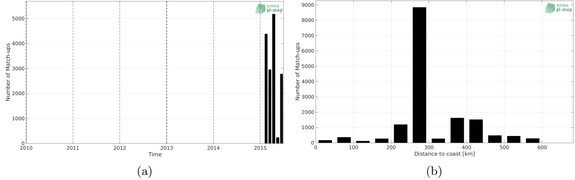
Figure 1: Number of match-ups between TSG (SAMOS) and Aquarius SSS L2 CAP v5 (JPL) SSS as a function of time (a) and as function of the distance to coast (b) over the Indian Ocean Pi-MEP region and for the full satellite product period.
