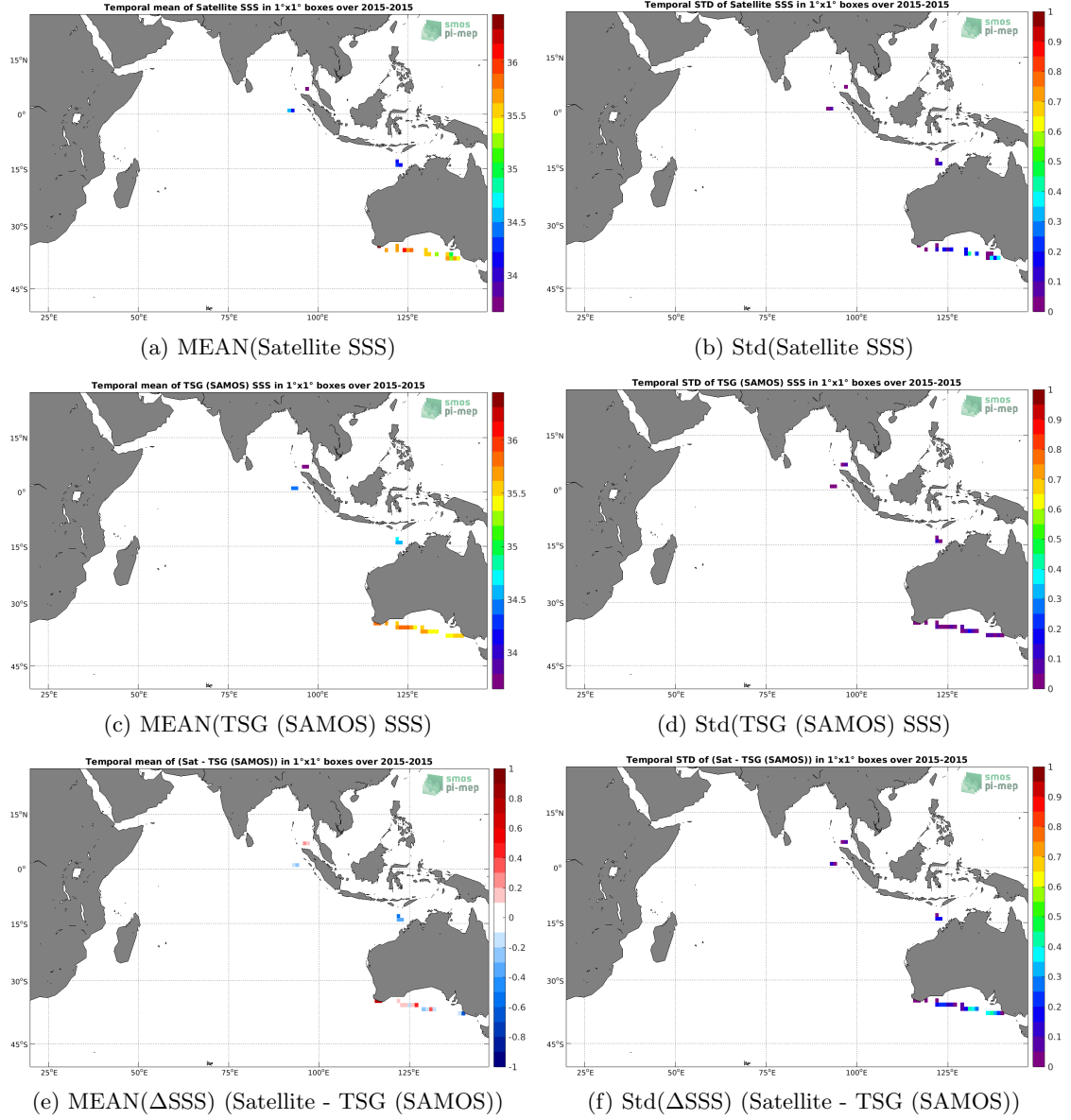
Figure 6: Temporal mean (left) and Std (right) of SSS from Aquarius SSS L2 CAP v5 (JPL) (top), TSG (SAMOS) (middle), and of \Delta SSS (Satellite - TSG (SAMOS)). Only match-up pairs are used to generate these maps.
