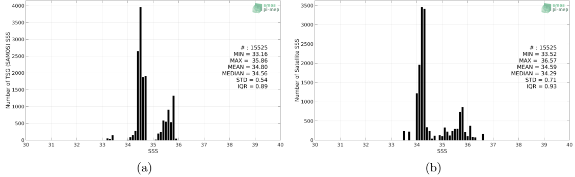
Figure 2: Histograms of SSS from TSG (SAMOS) (a) and Aquarius SSS L2 CAP v5 (JPL) (b) considering all match-up pairs per bins of 0.1 over the Indian Ocean Pi-MEP region and for the full satellite product period.
