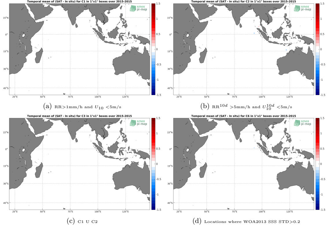
Figure 12: Temporal mean gridded over spatial boxes of size 1^\circ \times 1^\circ of \Delta SSS (Aquarius-L2-JPL-V5 - TSG-SAMOS) for 4 different subdatasets corresponding to: RR > 1\text{mm/h} and U_{10} < 5\text{m/s} (a), RR^{10d} > 5\text{mm/h} and U_{10}^{10d} < 5\text{m/s} (b), C1 U C2 (c), Locations where WOA2013 SSS STD > 0.2 (d).
