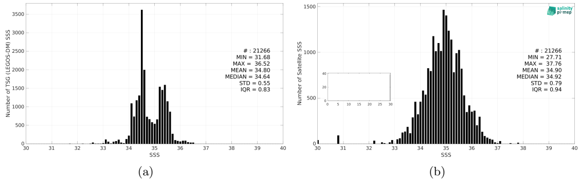
Figure 3: Histograms of SSS from TSG (LEGOS-DM) (a) and Aquarius SSS L2 CAP v5 (JPL) (b) considering all match-up pairs per bins of 0.1 over the Indian Ocean Pi-MEP region and for the full satellite product period.
