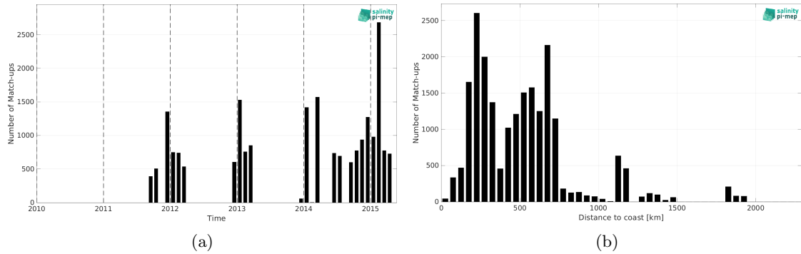
Figure 2: Number of match-ups between TSG (LEGOS-DM) and Aquarius SSS L2 CAP v5 (JPL) SSS as a function of time (a) and as function of the distance to coast (b) over the Indian Ocean Pi-MEP region and for the full satellite product period.
