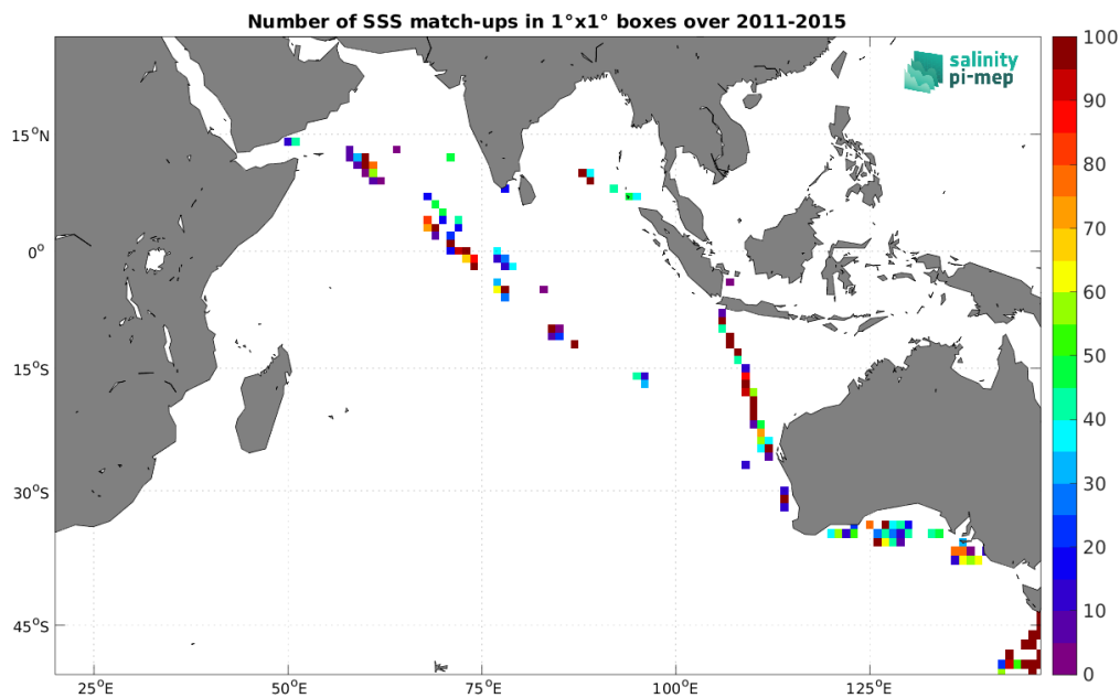
Figure 5: Number of SSS match-ups between TSG (LEGOS-DM) SSS and the Aquarius SSS L2 CAP v5 (JPL) SSS product for the Indian Ocean Pi-MEP region over 1^\circ \times 1^\circ boxes and for the full satellite product period.
